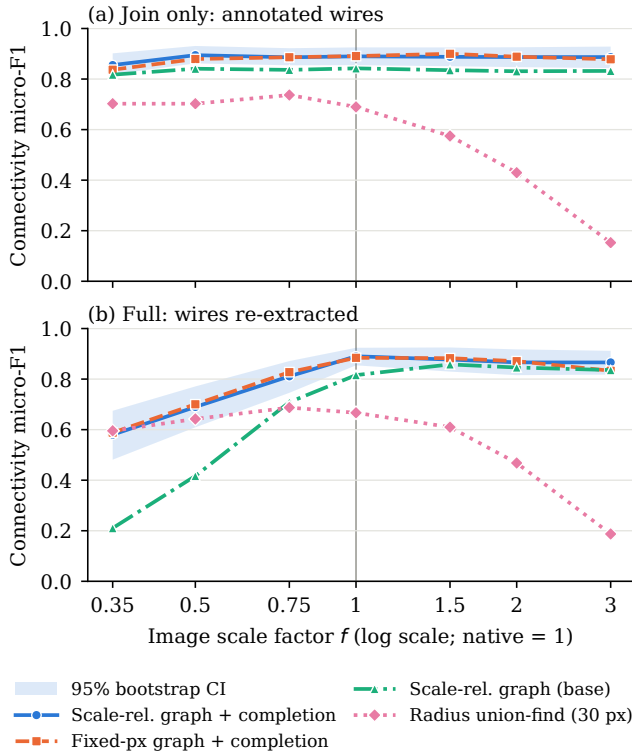
Fig. 8. Component-pair micro-F1 on the 31 images resampled by factor f (native f = 1 ). (a) Join only, with annotated wires rescaled with the image. (b) Full pipeline, with wires re-extracted from each rescaled image. Components are annotated boxes in both panels; shaded bands are 95% bootstrap CIs for our join.
