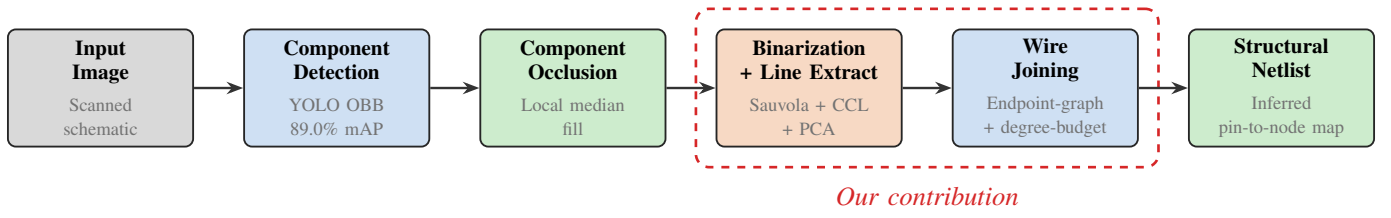
Fig. 1. Pipeline for structural circuit-netlist recovery. The highlighted stages extract wire endpoints and join them into nets.
