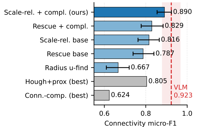
Fig. 7. Micro-averaged component-pair F1 on the 31-image human-verified benchmark with annotated component boxes and detected wires. Error bars are 95% bootstrap CIs; the dashed line marks the VLM reference (Claude Opus 4.8).
