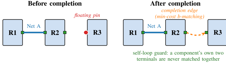
Fig. 4. Degree-budget completion. Left: after base joining, some pins are floating (connected only to their own component). Right: completion reconnects floating pins by min-cost b -matching (orange dashed); a guard rejects merges between nets that already share a component.
