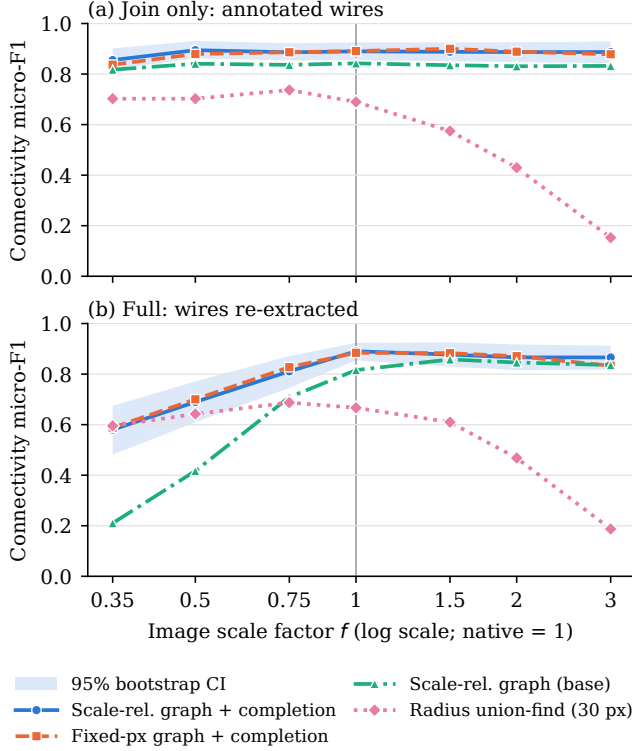
Fig. 8. Component-pair micro-F1 on the 31 images resampled by factor f (native f = 1 ). (a) Join only, with annotated wires rescaled with the image. (b) Full pipeline, with wires re-extracted from each rescaled image. Components are annotated boxes in both panels; shaded bands are 95% bootstrap CIs for our join.
