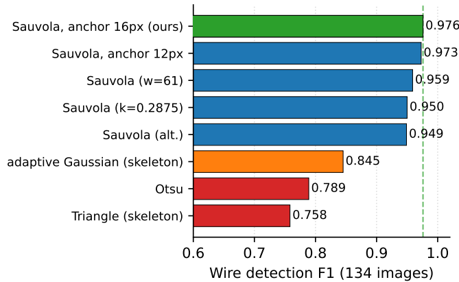
Fig. 6. Wire detection F1 across thresholding methods and pipeline variants (134 images, annotated component boxes). The adaptive Gaussian and Triangle bars use skeleton extraction (F1 = 0.845 and 0.758).
