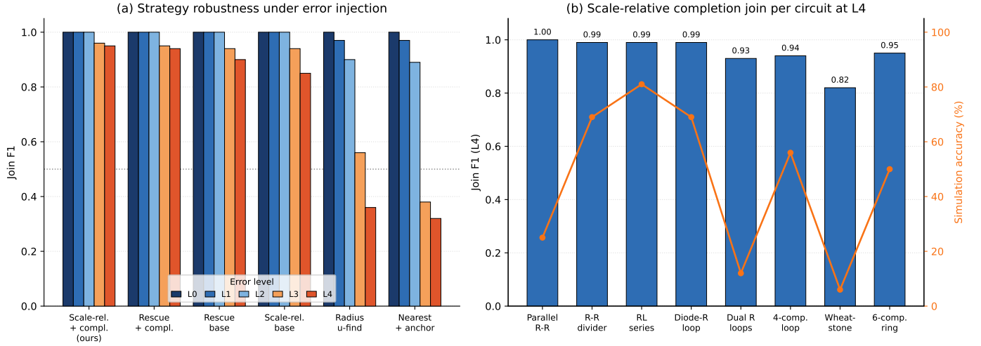
Fig. 5. (a) Join strategies under error injection (15 circuits \times 8 seeds): mean component-pair F1 at each severity level (L0–L4, dark to light to red). (b) The scale-relative completion join per circuit at L4 (16 seeds): bars are component-pair F1, the orange line is simulation accuracy.
