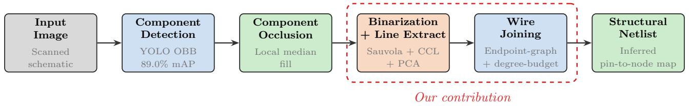
FIGURE 1. Pipeline for structural circuit-netlist recovery. The highlighted stages extract wire endpoints and join them into nets.
