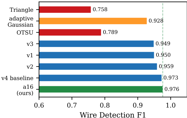
Wire Detection (134 images)
