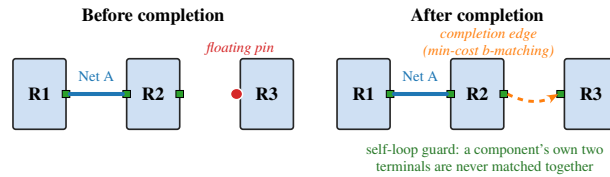
FIGURE 4. Degree-budget completion. Left: after base joining , some pins are floating (connected only to their own component). Right: completion reconnects floating pins by min-cost b -matching (orange dashed); a guard rejects merges between nets that already share a component .
