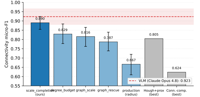
Fig. 7. Micro-averaged connectivity F1 on the 31-image human-verified net-level benchmark (component-pair metric). Our scale-relative completion join leads all deterministic strategies and the classical Hough and connected-component baselines (run on identical detected wires). The dashed line marks a strong VLM evaluated on the same 31 images, from which our join is statistically indistinguishable (paired micro-F1 difference +0.033, 95% bootstrap CI [-0.009, +0.078] ) while being deterministic, simulatable, and orders of magnitude cheaper. Error bars are 95% bootstrap CIs.
