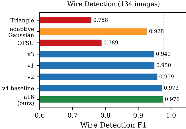
Fig. 5. Wire detection F1 across thresholding methods and pipeline variants (134 images). Our configuration (a16) achieves F1 = 0.976. OTSU and triangle thresholding degrade significantly.
