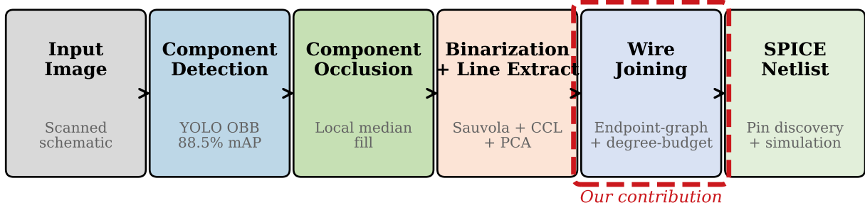
Fig. 1. End-to-end pipeline for scanning circuit diagram digitization. Our contributions focus on the wire joining stage (dashed red), which determines which extracted wire segments connect to which component pins.
