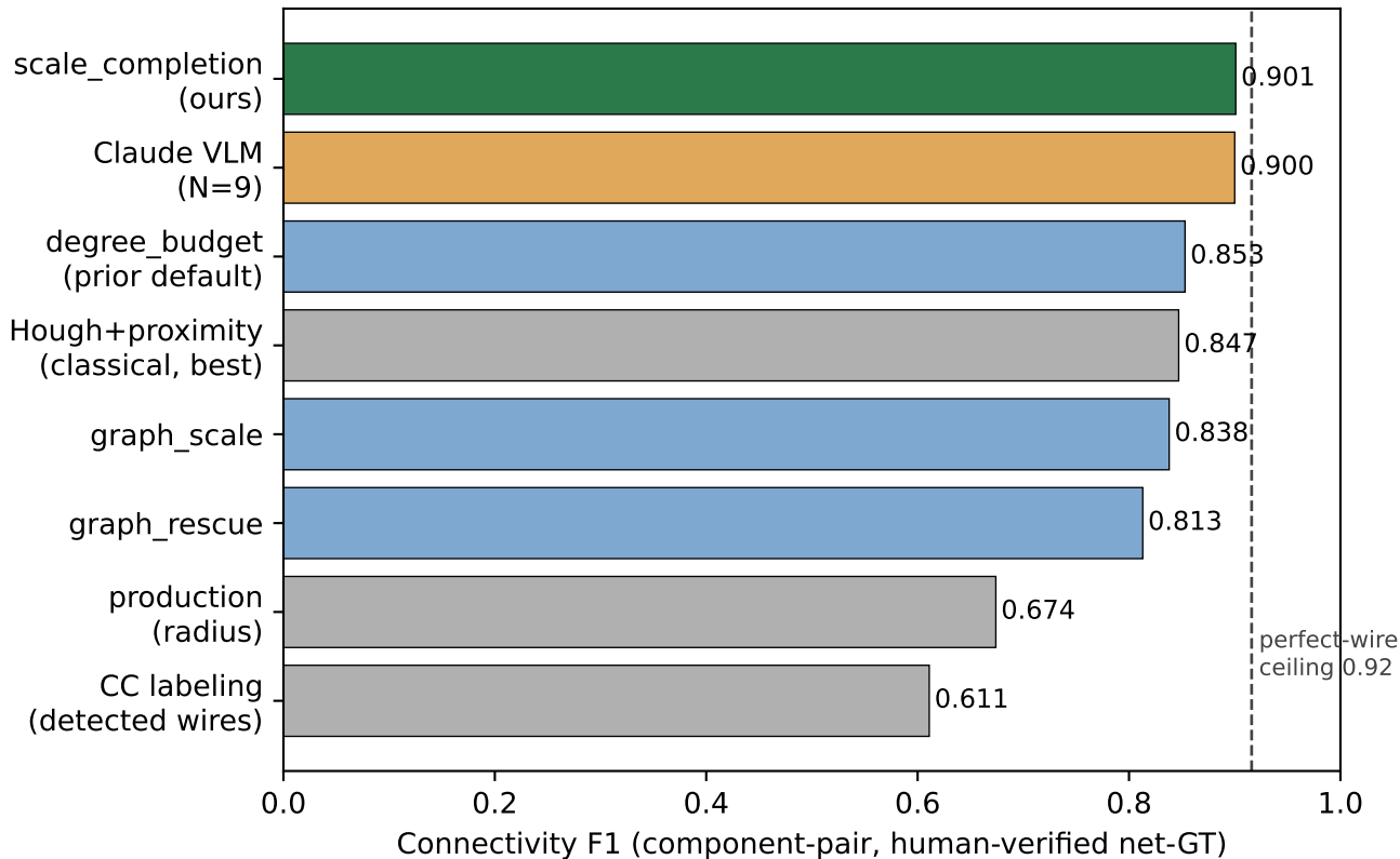
Real-image connectivity: ours vs join strategies, classical baselines, VLM
