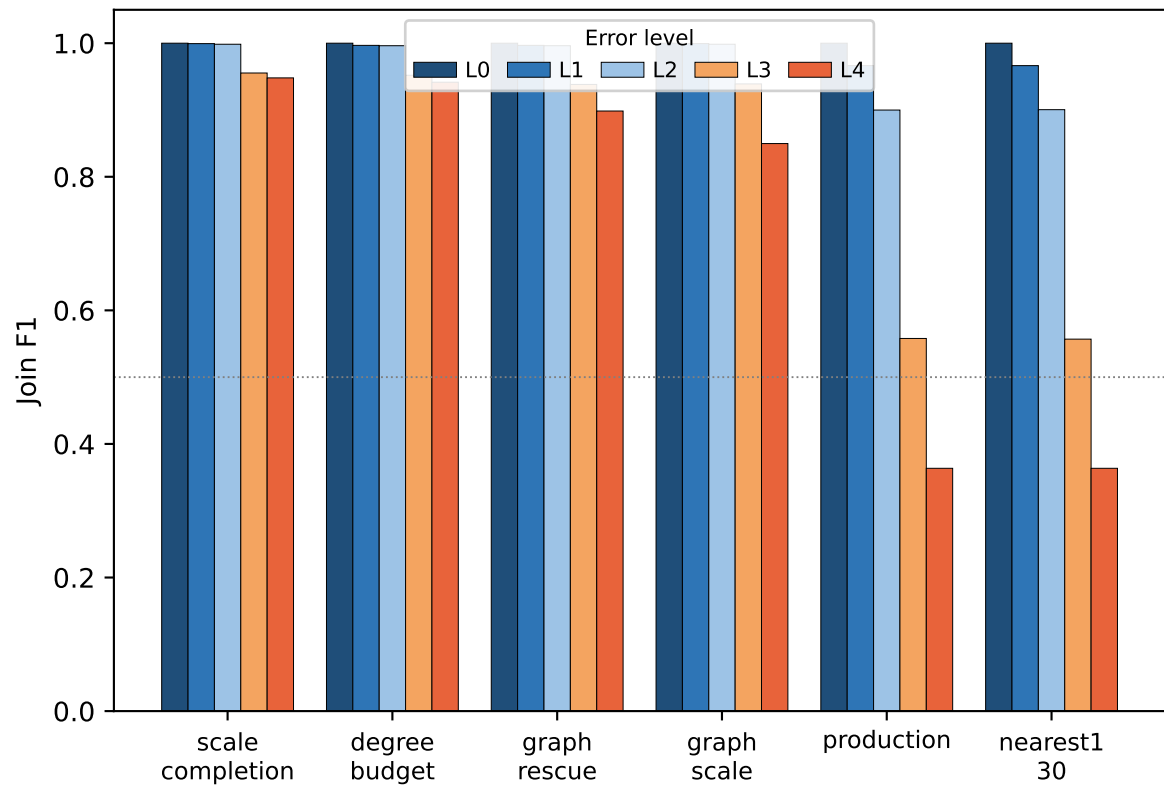
(a) Strategy robustness under error injection
