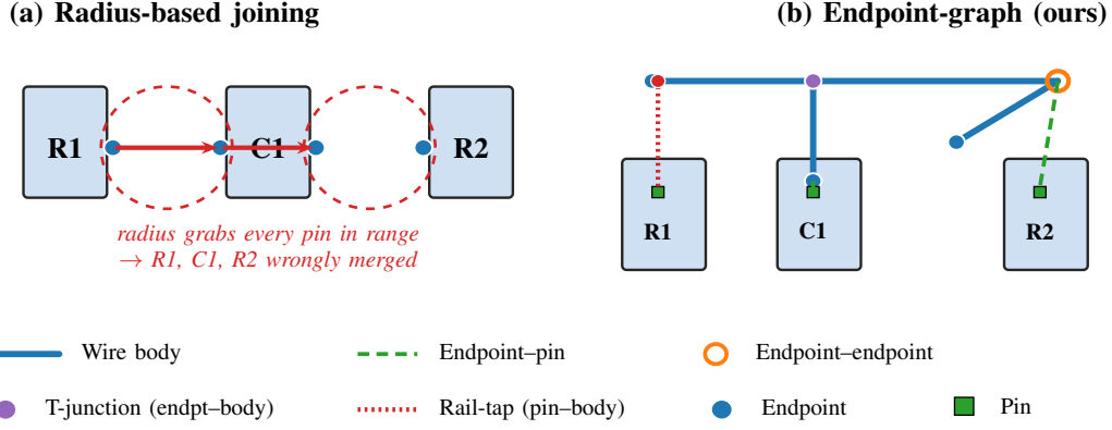
Fig. 3. Joining approaches compared. (a) Radius-based join (legacy): each wire endpoint grabs all pins within a fixed threshold, causing over-merging. (b) Our endpoint-graph model: typed edges and component-first pin assignment generate connectivity candidates, with directional scoring confined to the fallback pin search. Incorrect base merges remain possible.
