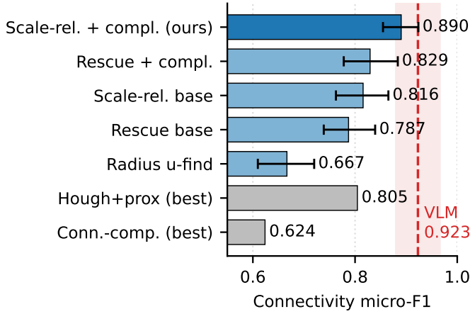
Fig. 7. Micro-averaged connectivity F1 on the 31-image human-verified net-level benchmark (component-pair metric). The scale-relative completion join has the highest score among the evaluated deterministic configurations and classical baselines on these detected wires. The dashed line marks the VLM diagnostic (Claude Opus 4.8). Both methods receive annotated component boxes; the VLM-minus-join difference is +0.033 (95% bootstrap CI [-0.009, +0.078] ). The interval does not establish equivalence, cost superiority or a global validity guarantee. Error bars are 95% bootstrap CIs.
