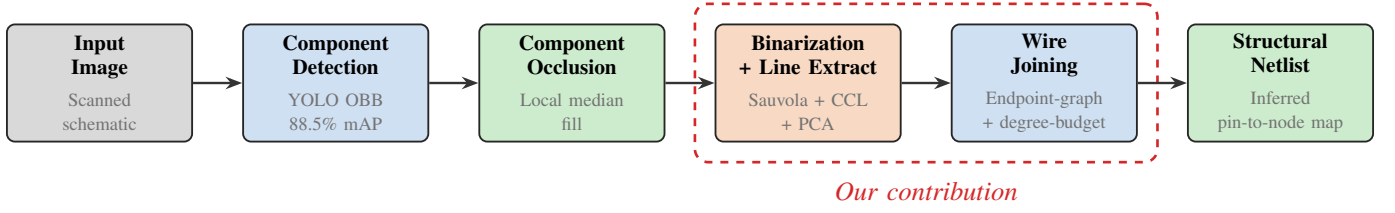
Fig. 1. Pipeline for structural circuit-netlist recovery. The highlighted stages extract wire endpoints and infer connectivity. The net-level experiments use annotated component boxes to isolate joining; they do not establish an end-to-end error hierarchy or validate illustrative SPICE export.
