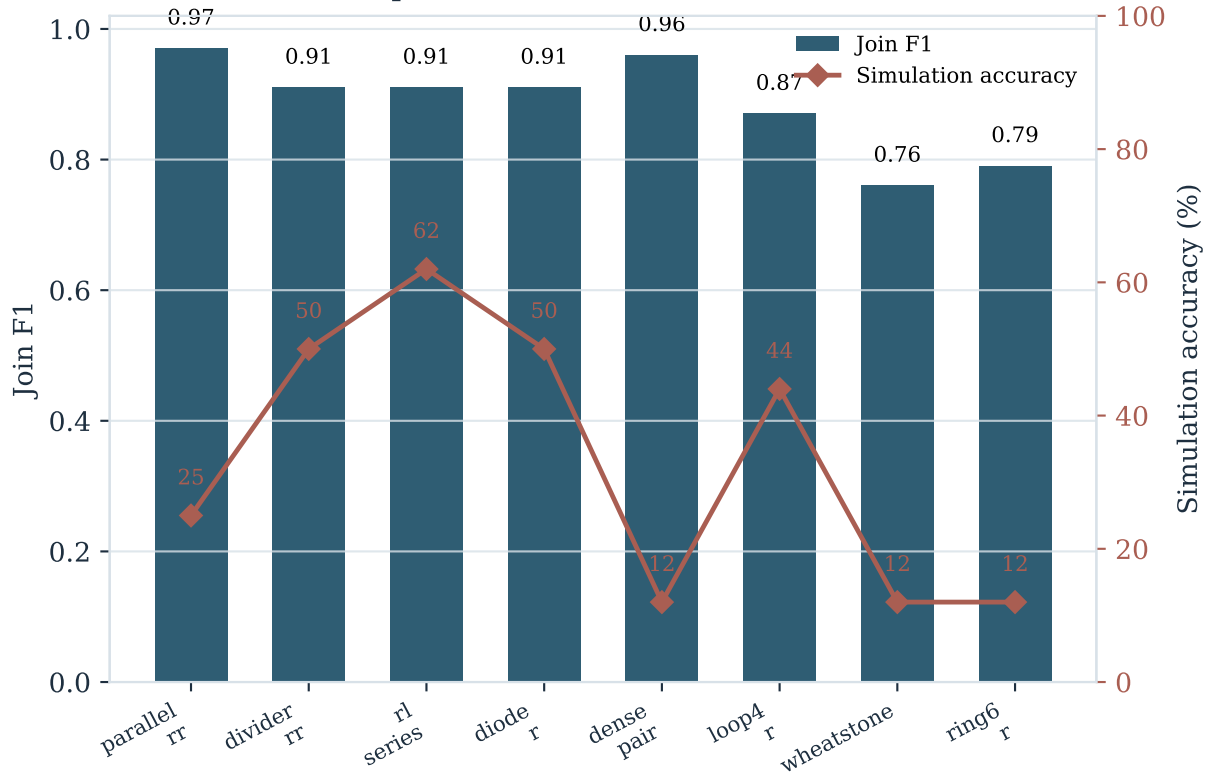
(b) Representative L4 circuit behavior
