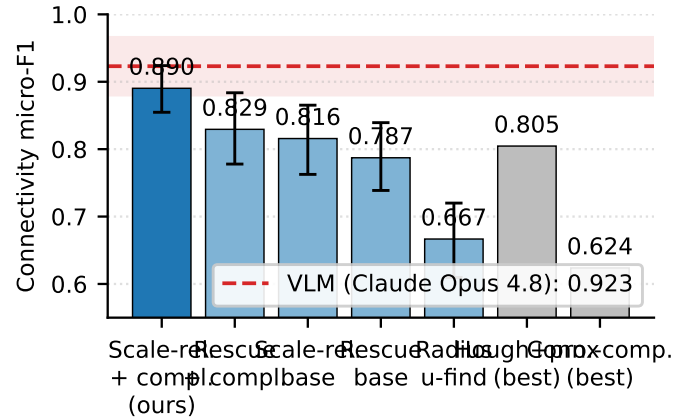
Fig. 7. Micro-averaged connectivity F1 on the 31-image human-verified net-level benchmark (component-pair metric). Our scale-relative completion join leads all deterministic strategies and the classical Hough and connected-component baselines (run on identical detected wires). The dashed line marks a strong VLM evaluated on the same 31 images, from which our join is statistically indistinguishable (paired micro-F1 difference +0.033, 95% bootstrap CI [-0.009, +0.078] ) while being deterministic, simulatable, and orders of magnitude cheaper. Error bars are 95% bootstrap CIs.
