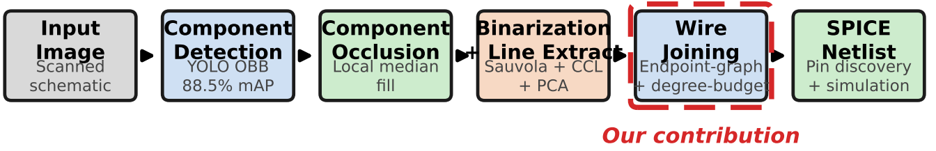
Fig. 1. End-to-end pipeline for scanning circuit diagram digitization. Our contributions focus on the wire joining stage (dashed red), which determines which extracted wire segments connect to which component pins.
