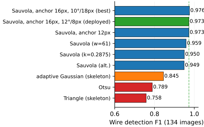
Fig. 6. Wire detection F1 across thresholding methods and pipeline variants (134 images, annotated component boxes). The green bar is the deployed extractor (12°/8 px deduplication, F1 0.973), used in all other experiments; the top bar is the best of 36 variants (10°/18 px, F1 0.976). The adaptive Gaussian and Triangle bars use skeleton extraction (F1 = 0.845 and 0.758).
