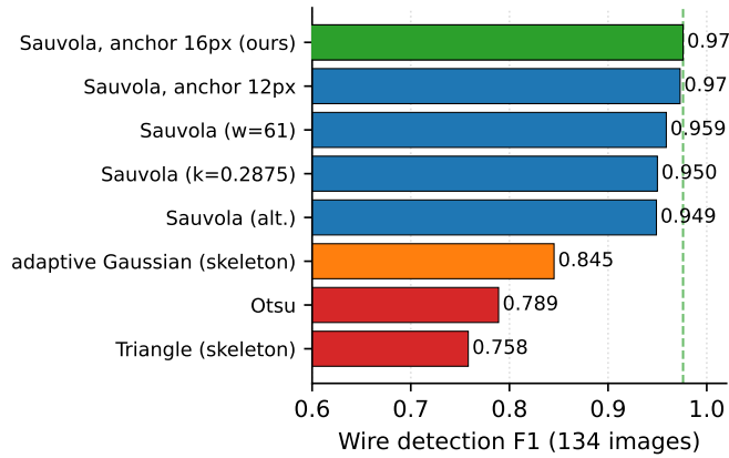
Fig. 6. Wire detection F1 across thresholding methods and pipeline variants (134 images, annotated component boxes). The adaptive Gaussian and Triangle bars use skeleton extraction (F1 = 0.845 and 0.758).
