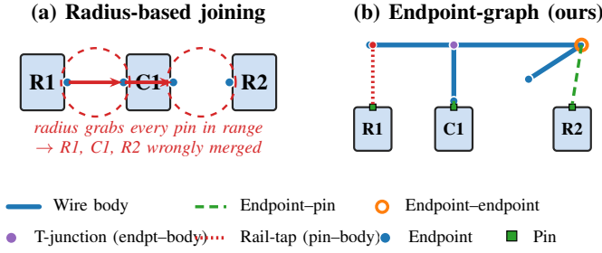
Fig. 3. Joining approaches compared. (a) Radius-based join (legacy): each wire endpoint grabs all pins within a fixed threshold, causing over-merging. (b) Our endpoint-graph model: typed edges (wire body, endpoint-pin) with directional preference resolve connectivity without over-merging.
