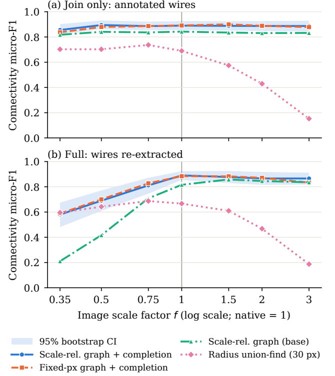
Fig. 8. Component-pair micro-F1 on the 31 images resampled by factor f (native f = 1 ). (a) Join only, with annotated wires rescaled with the image. (b) Full pipeline, with wires re-extracted from each rescaled image. Components are annotated boxes in both panels; shaded bands are 95% bootstrap CIs for our join.
