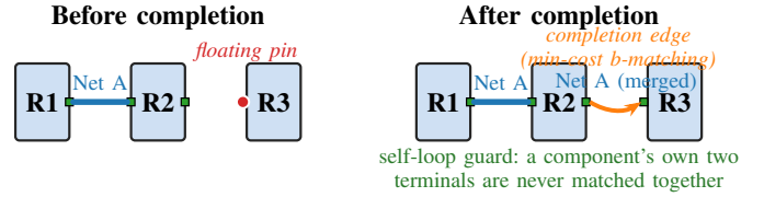
Fig. 4. Degree-budget completion. Left: After base joining, some pins are “floating” (touching only their own component). Right: Completion reconnects floating pins via min-cost b -matching (orange dashed), with self-loop guard preventing shorts within two-terminal components.
