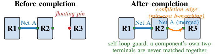
Fig. 4. Degree-budget completion. Left: After base joining, some pins are “floating” (touching only their own component). Right: Completion reconnects floating pins via min-cost b-matching (orange dashed), with self-loop guard preventing shorts within two-terminal components.
