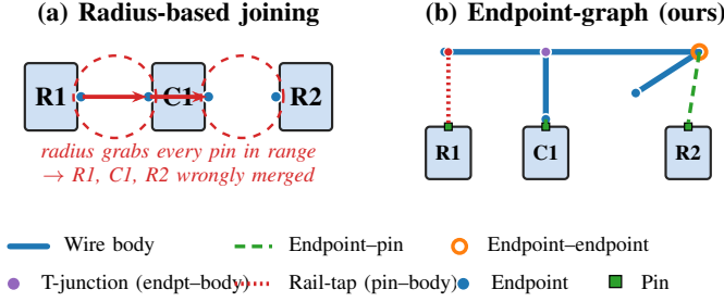
Fig. 3. Joining approaches compared. (a) Production radius-based join: each wire endpoint grabs ALL pins within a fixed threshold, causing over-merging. (b) Our endpoint-graph model: typed edges (wire body, endpoint-pin) with directional preference resolve connectivity without over-merging.
