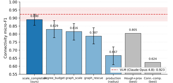
Fig. 7. Micro-averaged connectivity F1 on the 31-image human-verified net-level benchmark (component-pair metric). Our scale_completion join leads all deterministic strategies and the classical Hough and connected-component baselines (run on identical detected wires). The dashed line marks a strong VLM evaluated on the same 31 images, from which our join is statistically indistinguishable (paired micro-F1 difference +0.033, 95% bootstrap CI [-0.009, +0.078] ) while being deterministic, simulatable, and orders of magnitude cheaper. Error bars are 95% bootstrap CIs.
