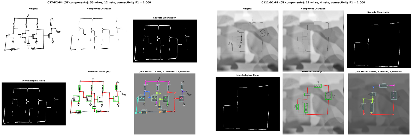
Fig. 2. Pipeline stages on two real hand-drawn circuit images, joined with our scale_completion strategy (connectivity F1 = 1.000 on both). Left: a four-transistor analog cell (35 wires, 12 nets); right: an RLC loop photographed on a textured surface (12 wires, 4 nets). Each panel shows, in order: original scan, component occlusion, Sauvola binarization, morphological close, detected wires (red overlay), and the join result. In the join result every recovered net is a distinct colour drawn along its conductors; component bounding boxes are the ground-truth labels (as used throughout the net-level evaluation, isolating the join), filled dots are device pins, diamonds mark junctions, and triangles mark terminals and ground.
