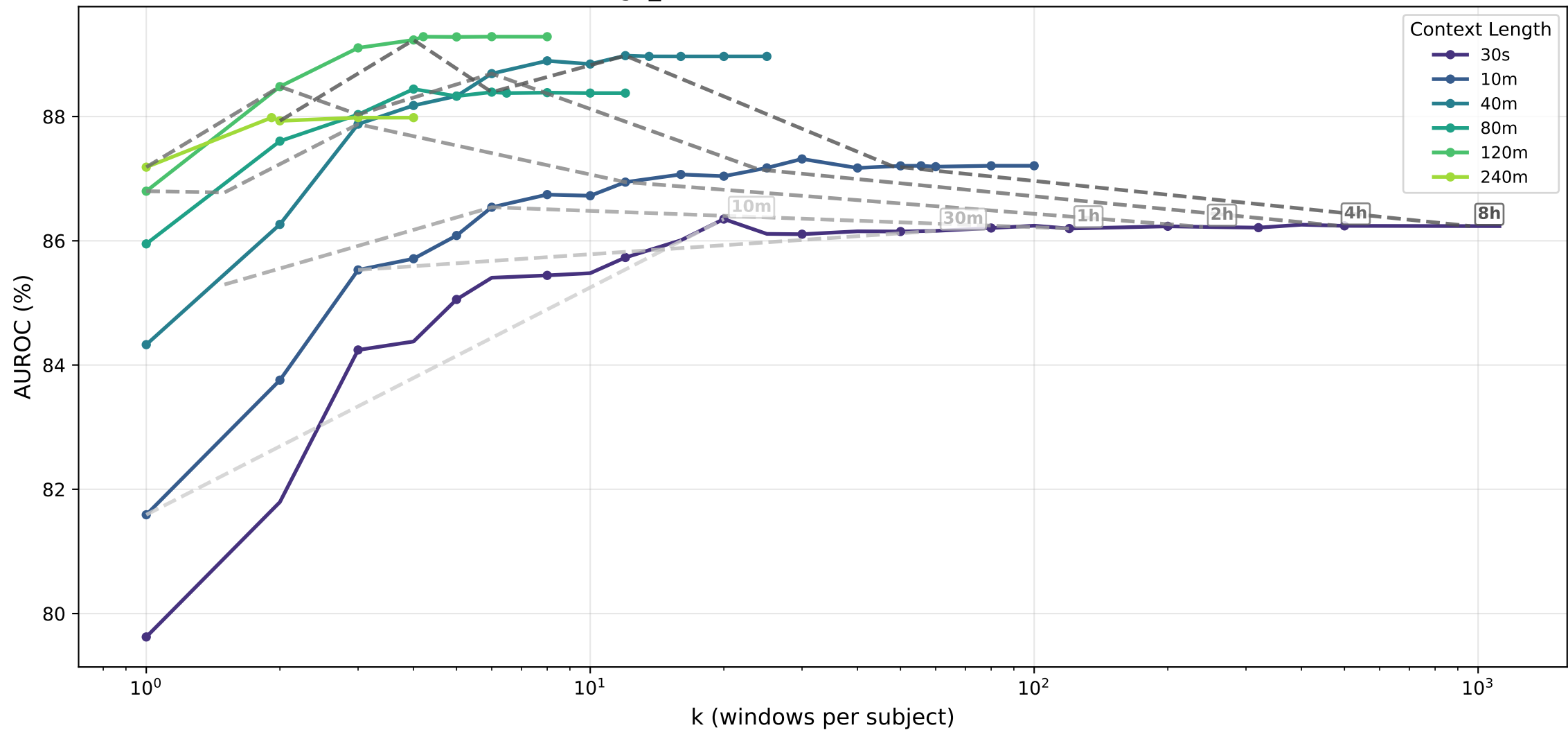
age_class · lstm — AUROC (%) vs k
