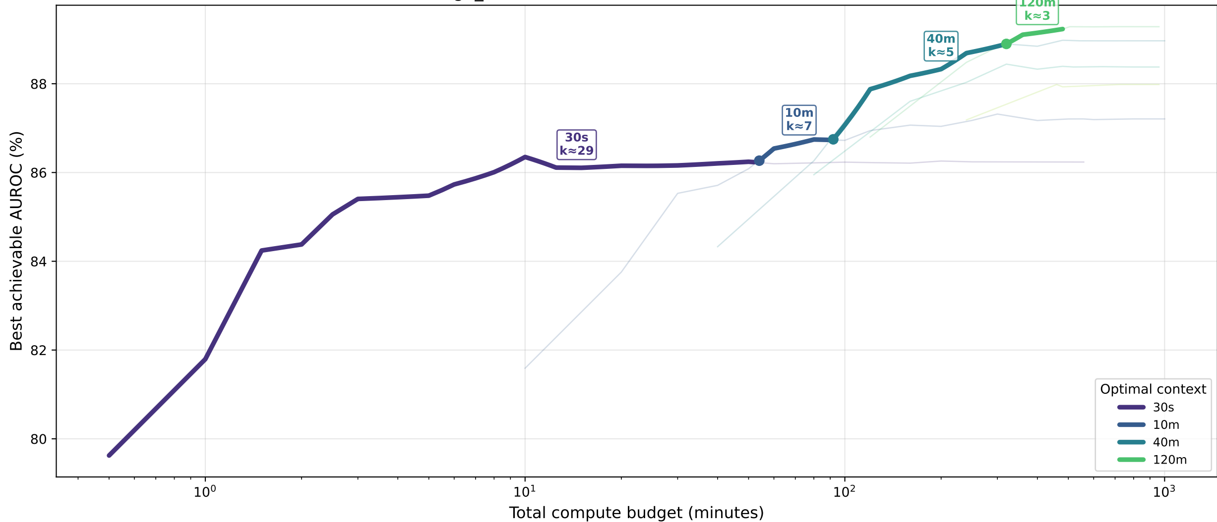
age_class · lstm — Pareto Front: AUROC (%)
