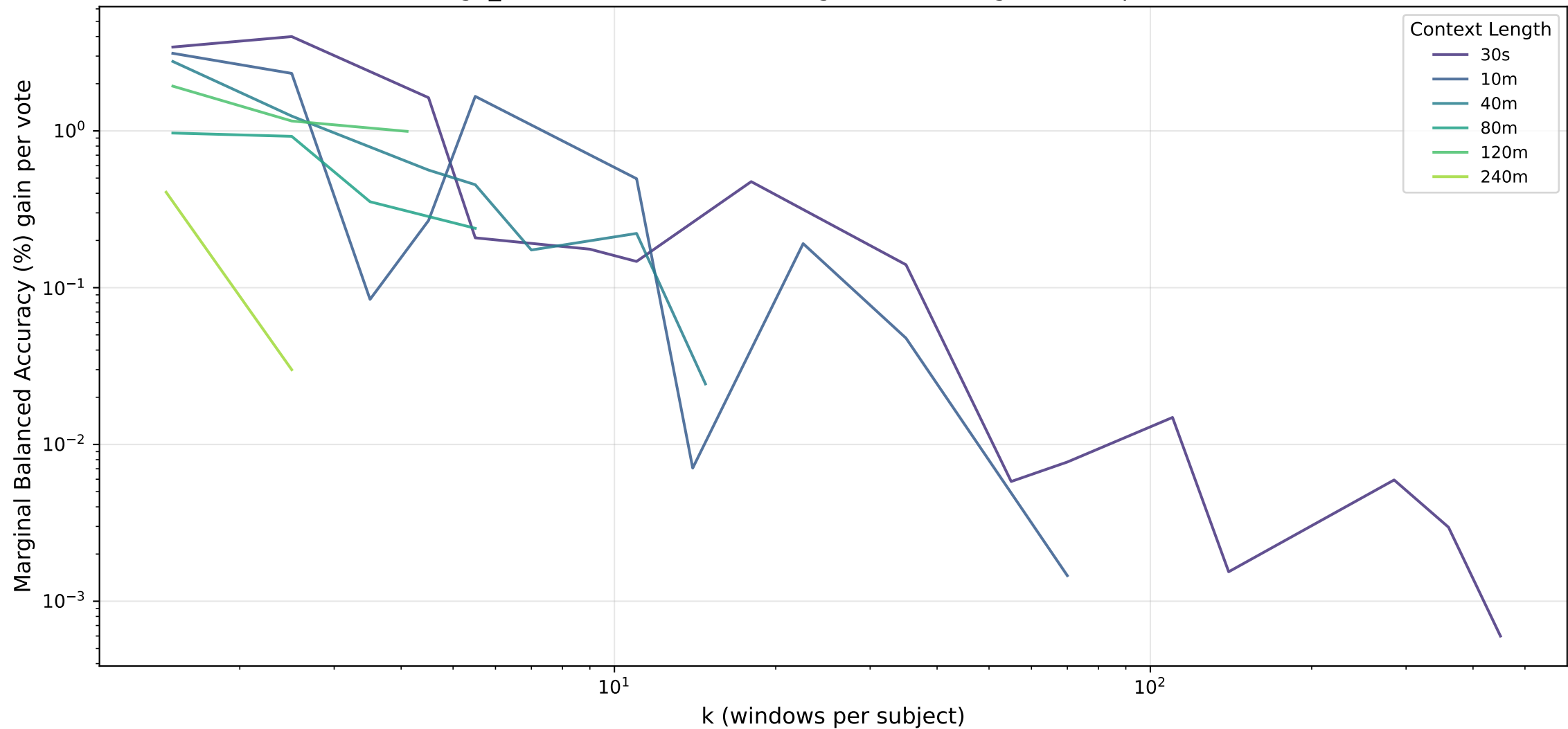
age_class · lstm — Diminishing Returns: Marginal Gain per Vote
