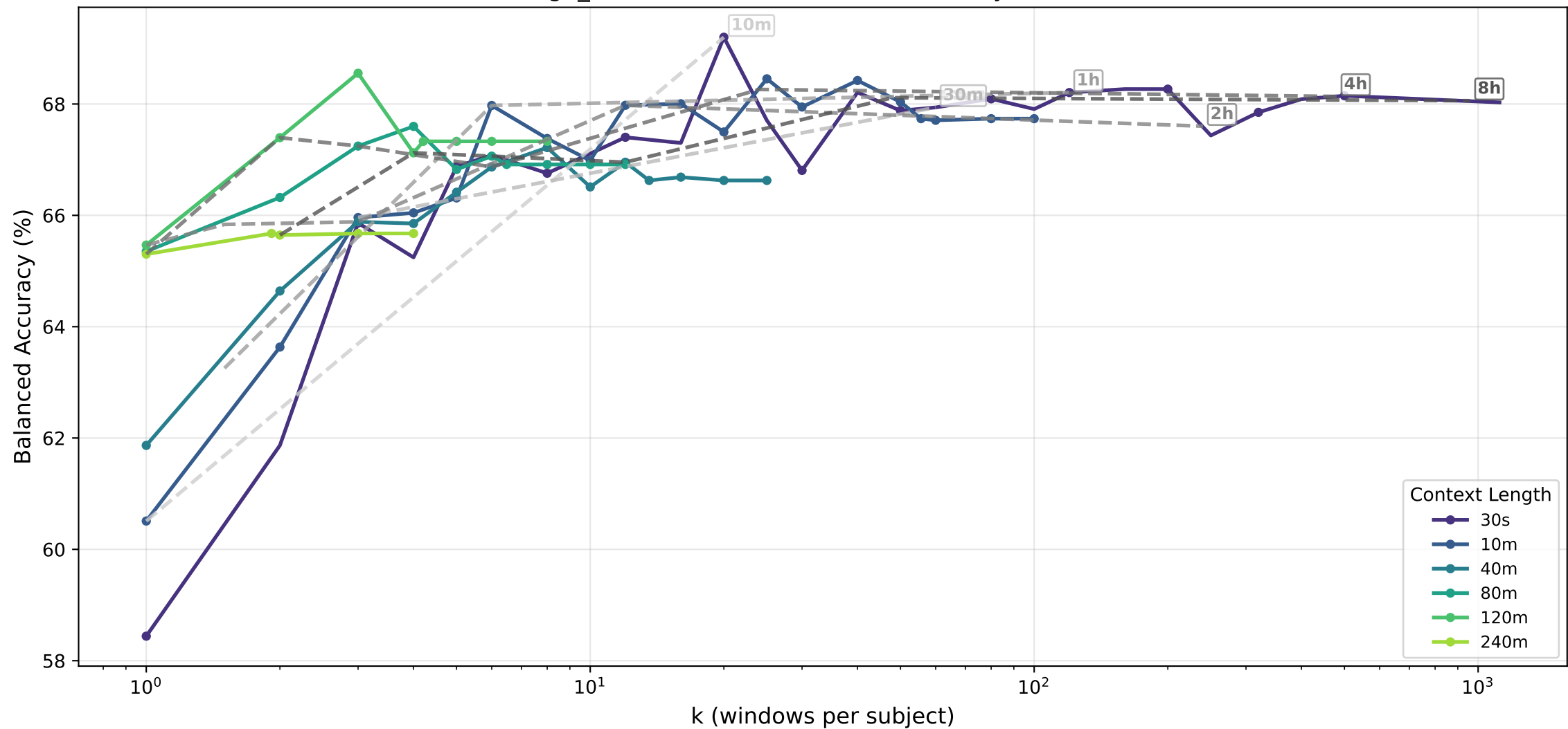
age_class · lstm — Balanced Accuracy (%) vs k
