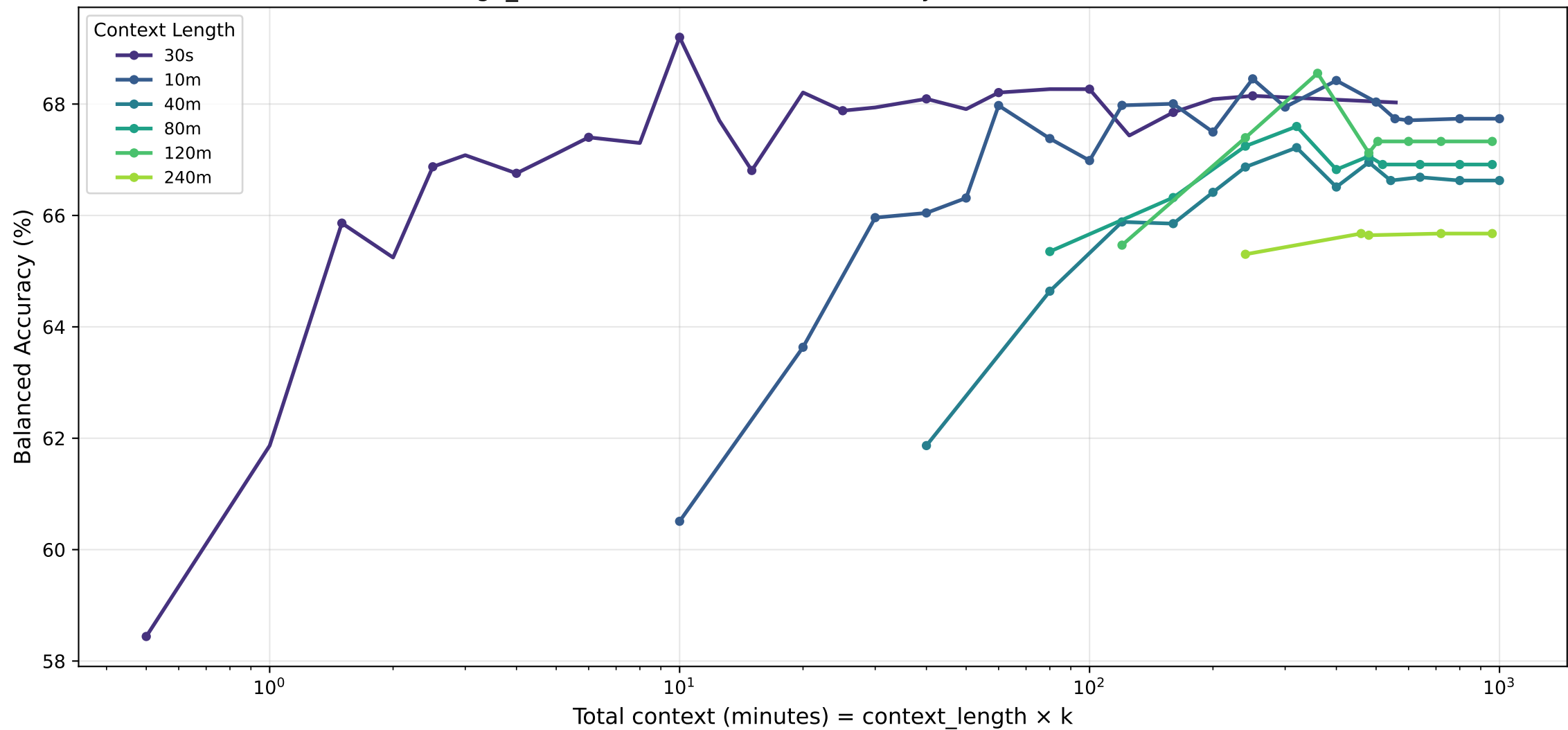
age_class · lstm — Balanced Accuracy (%) vs Total Context
