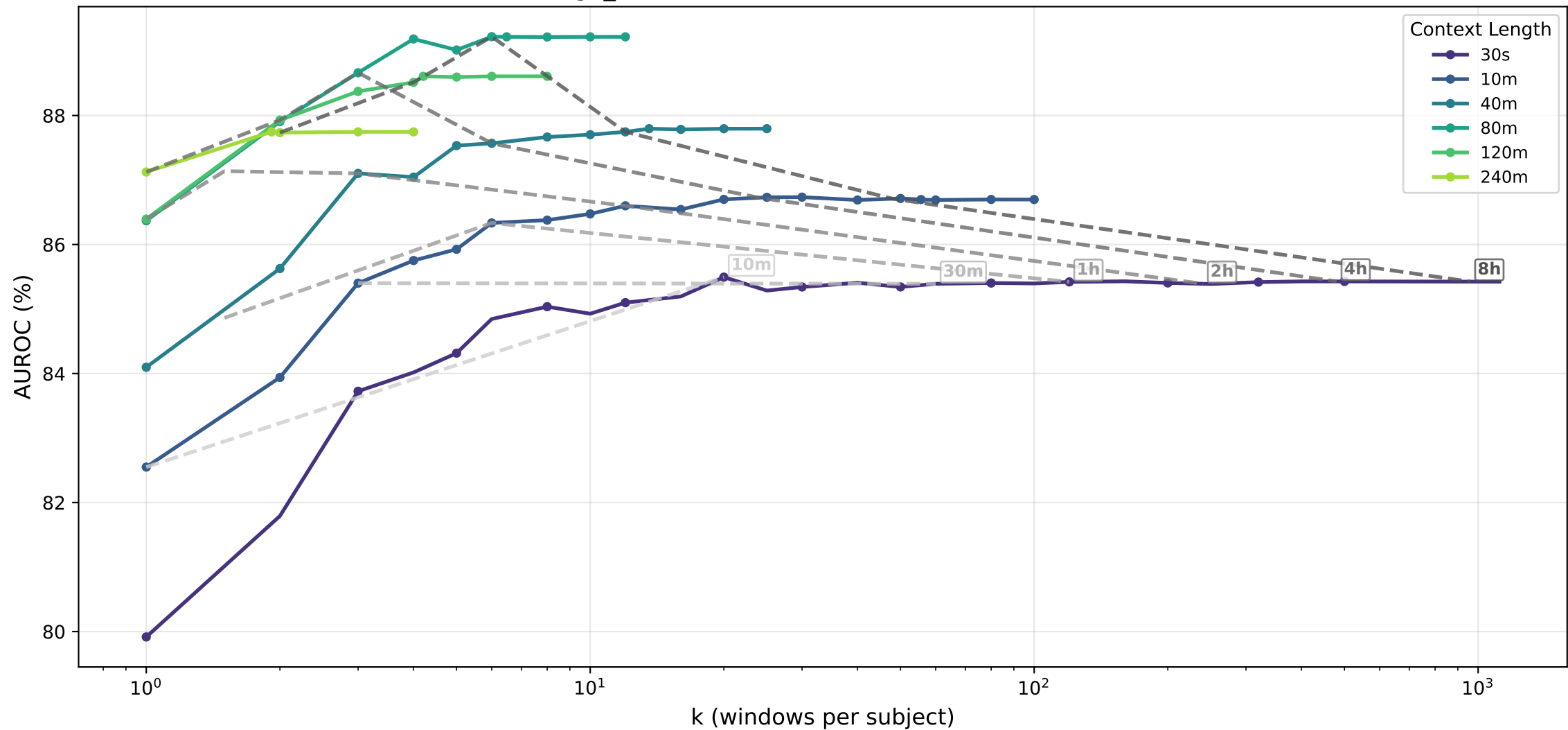
age_class · transformer — AUROC (%) vs k
