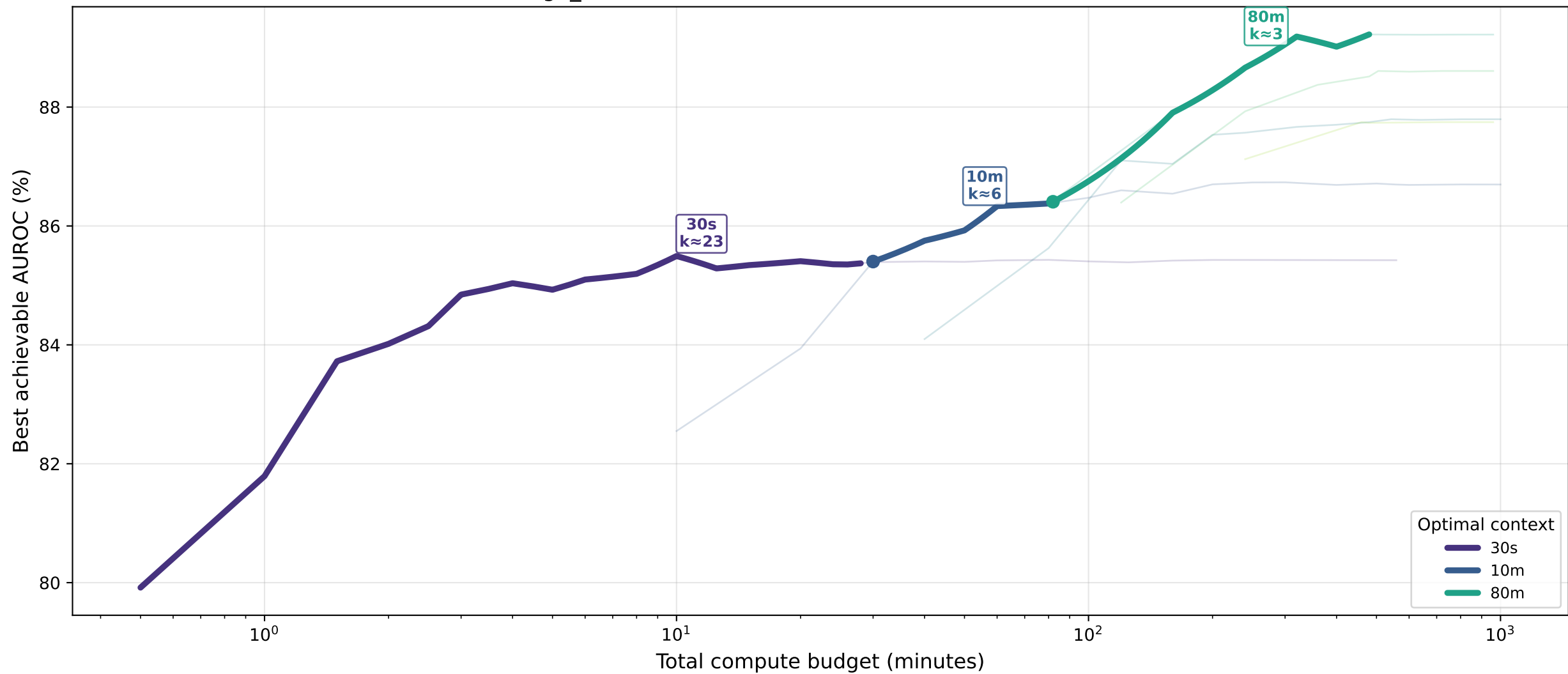
age_class · transformer — Pareto Front: AUROC (%)
