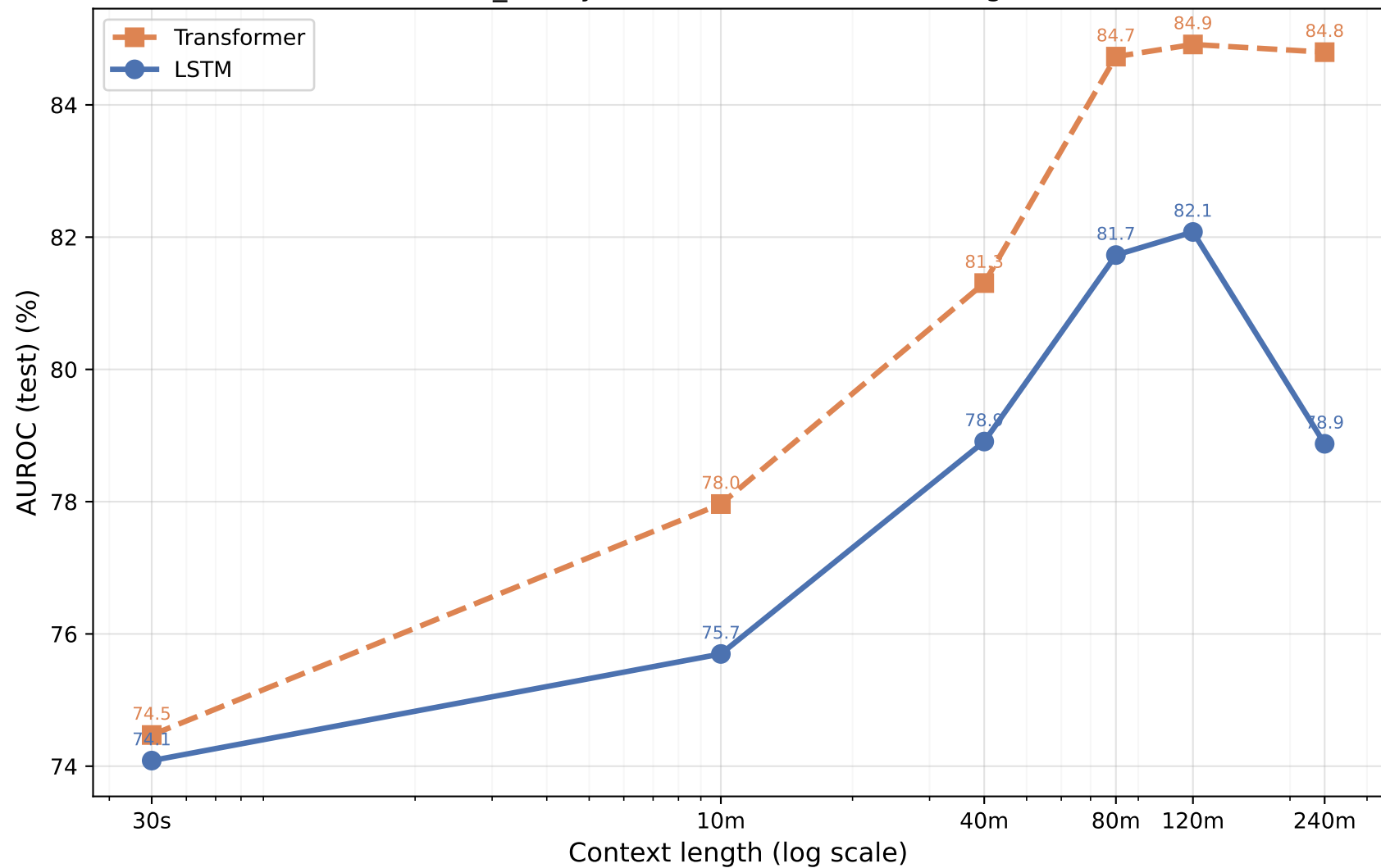
sex_binary — AUROC vs Context Length
