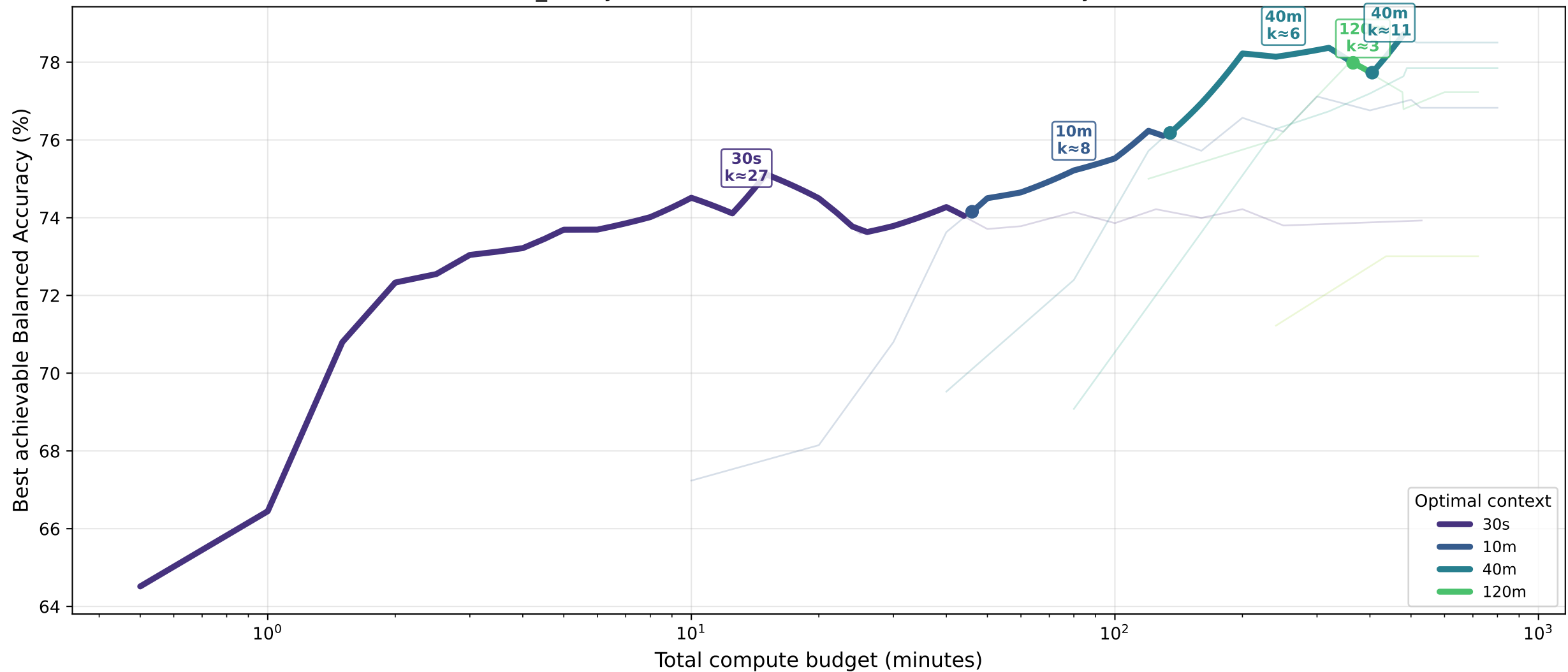
sex_binary · lstm — Pareto Front: Balanced Accuracy (%)
