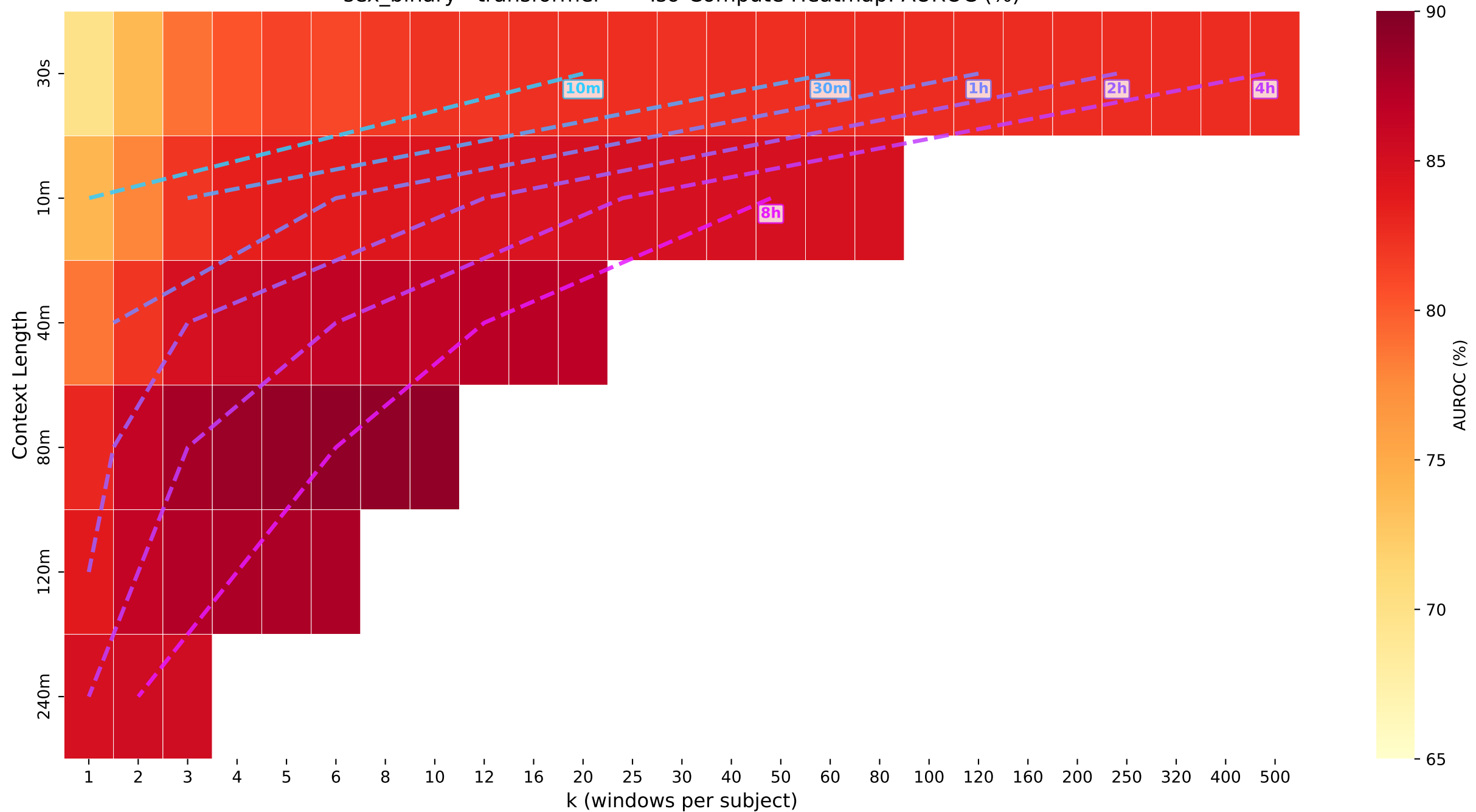
sex_binary · transformer — Iso-Compute Heatmap: AUROC (%)
