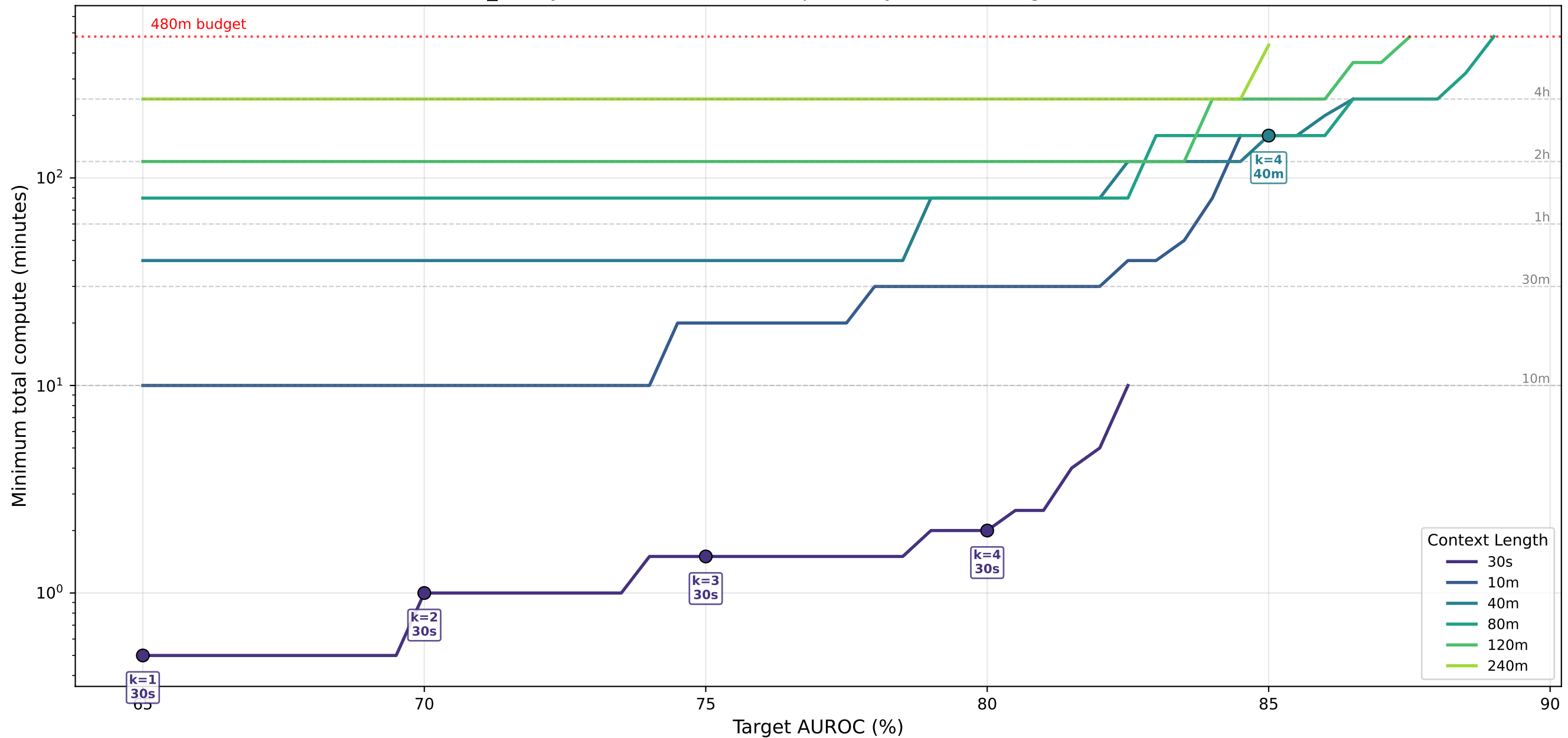
sex_binary · transformer — Cheapest Way to Reach Target AUROC (%)
