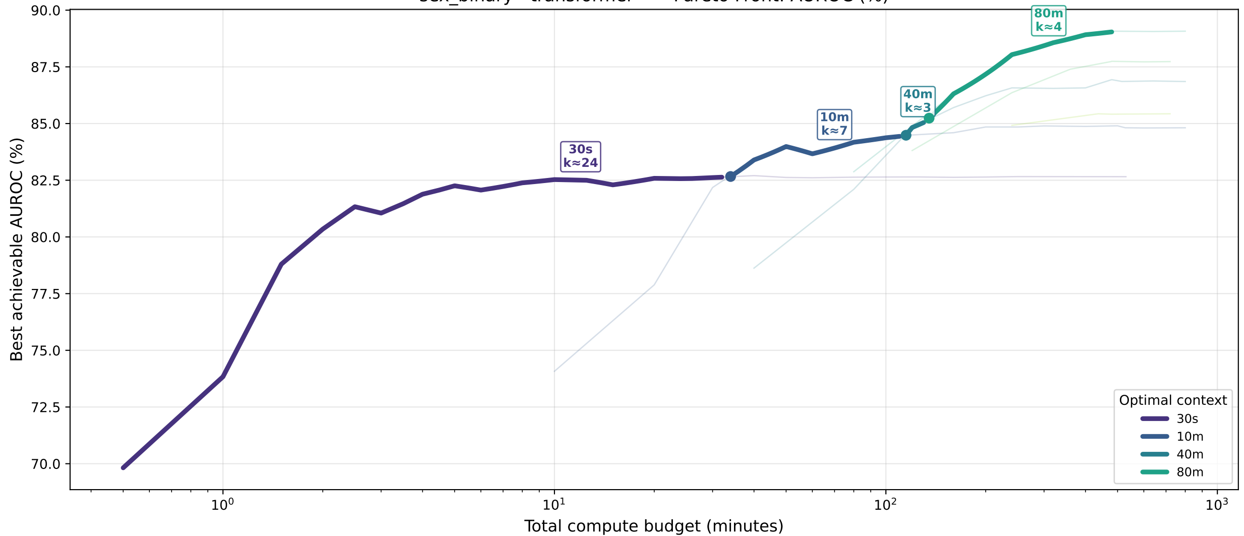
sex_binary · transformer — Pareto Front: AUROC (%)
