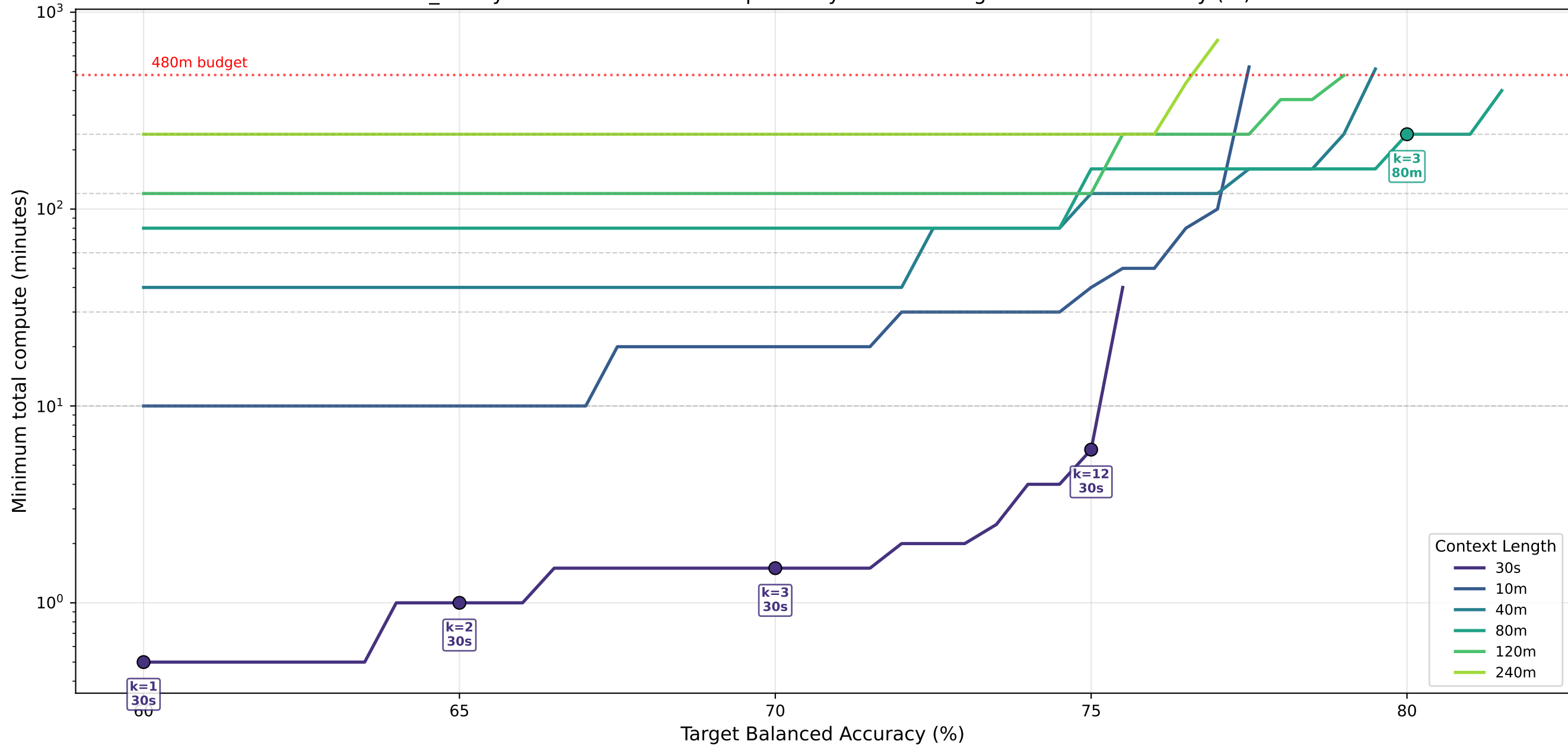
sex_binary · transformer — Cheapest Way to Reach Target Balanced Accuracy (%)
