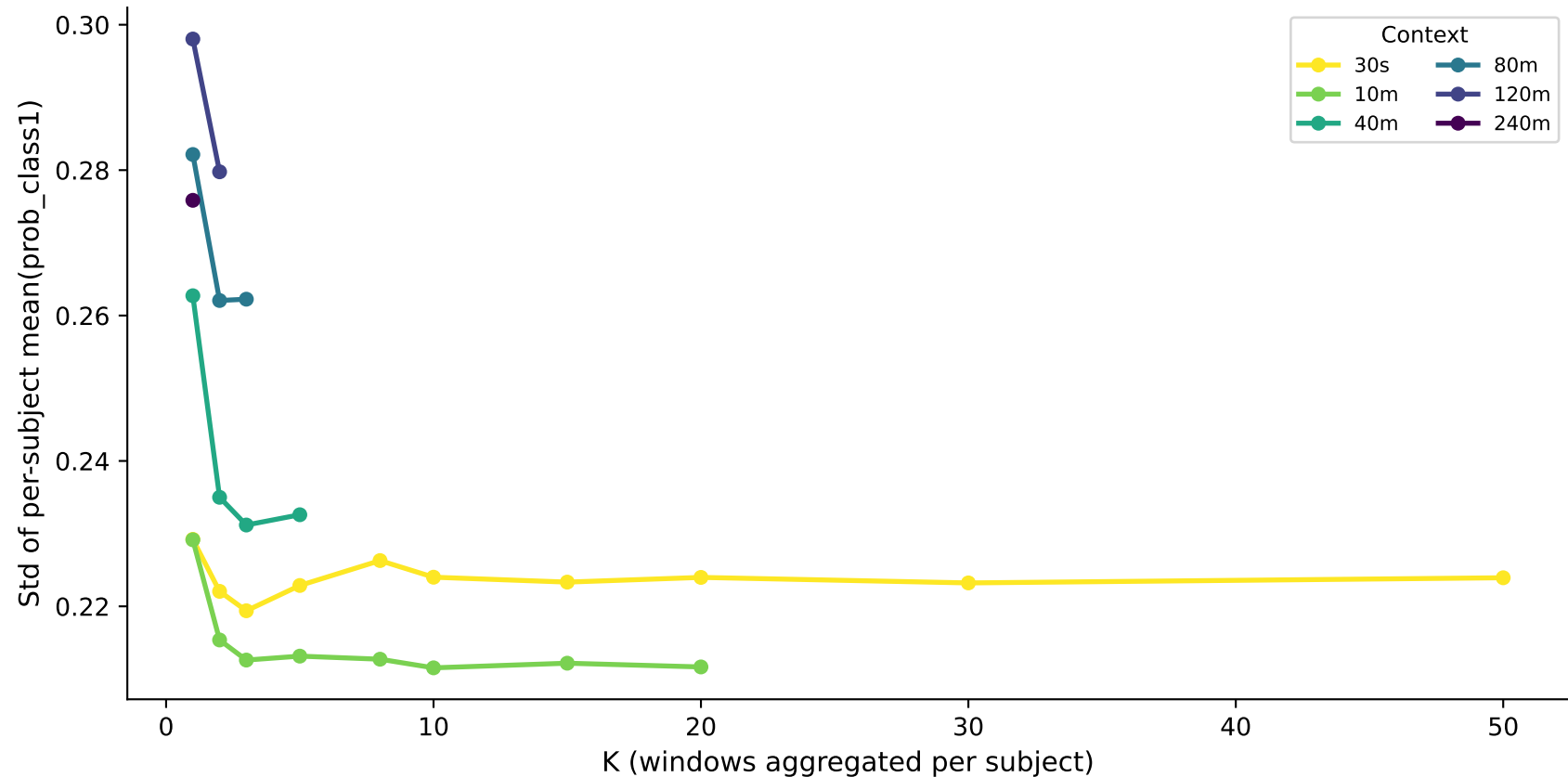
Prediction Variance vs K — age_class (LSTM) Aggregation stabilises predictions (lower std = more consistent)
