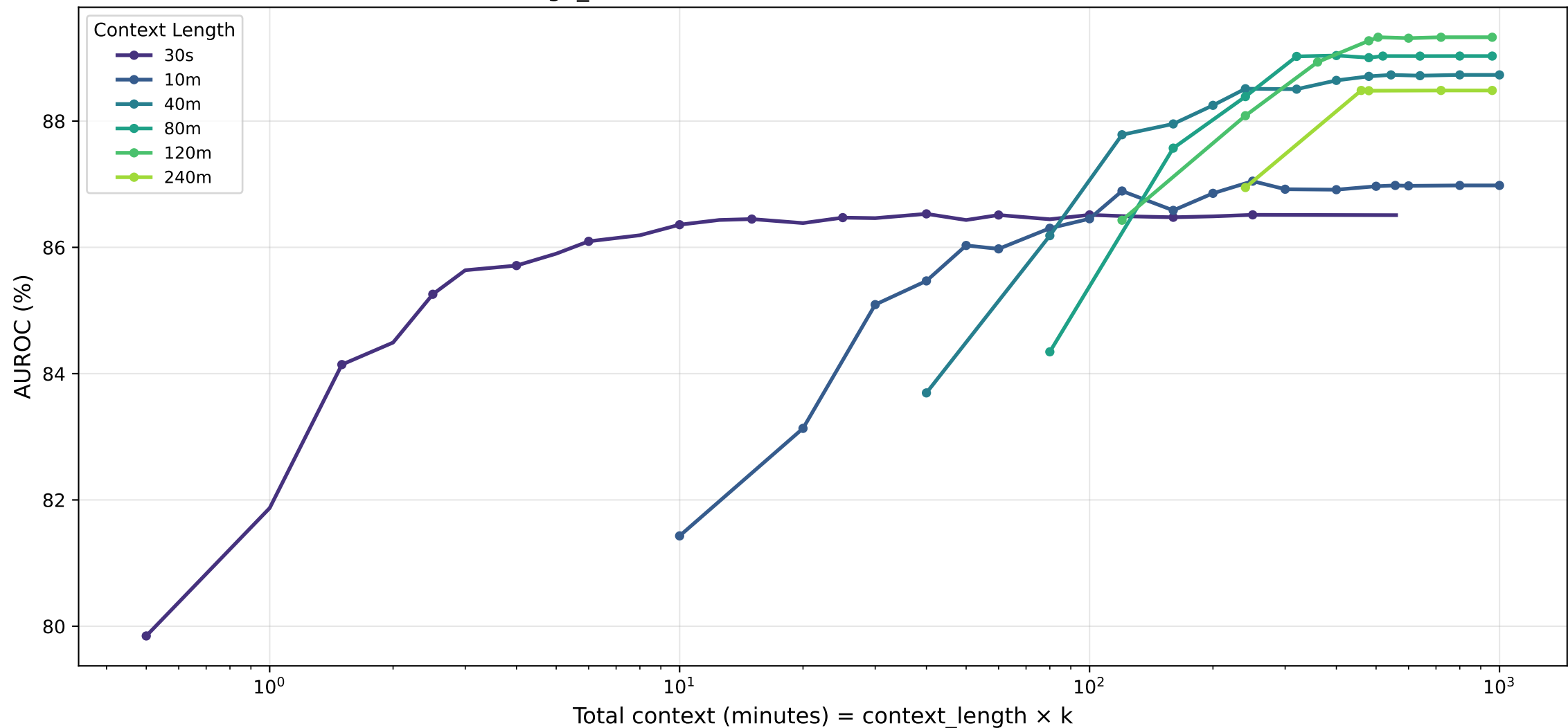
age_class · lstm — AUROC (%) vs Total Context
