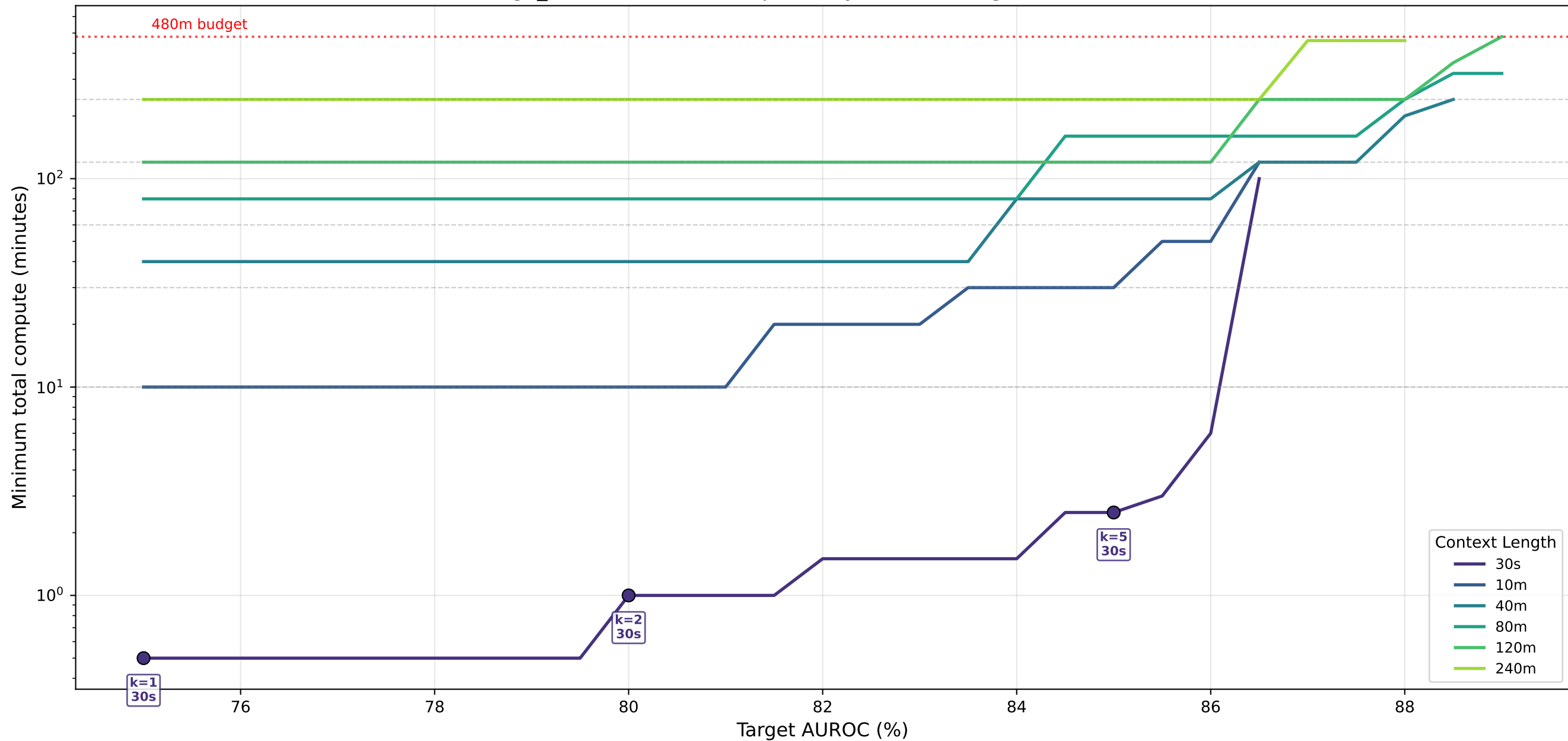
age_class · lstm — Cheapest Way to Reach Target AUROC (%)
