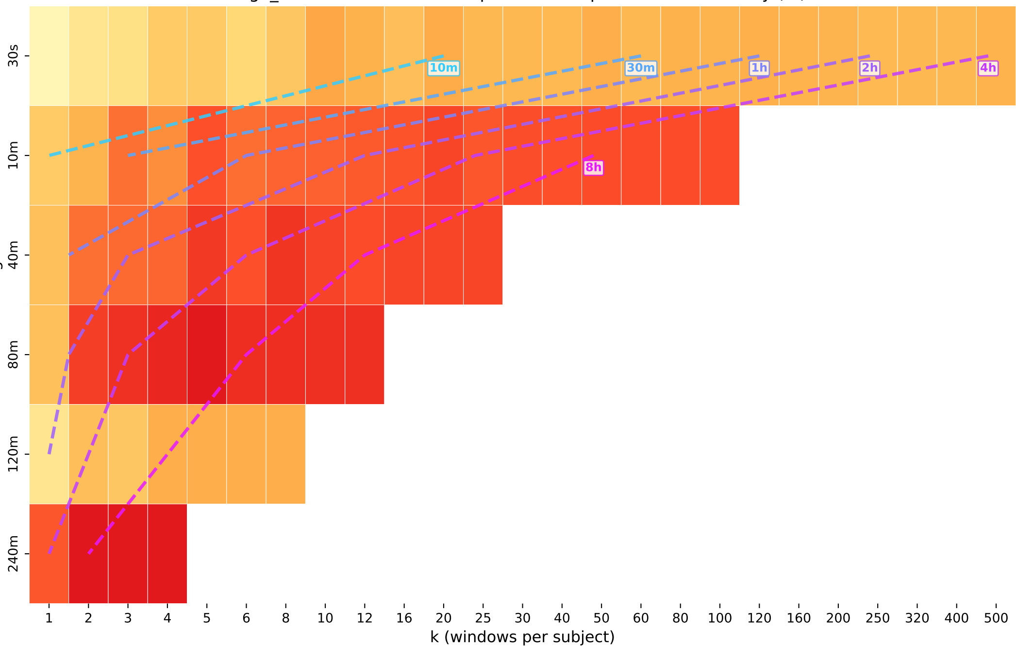
age_class · lstm — Iso-Compute Heatmap: Balanced Accuracy (%)
