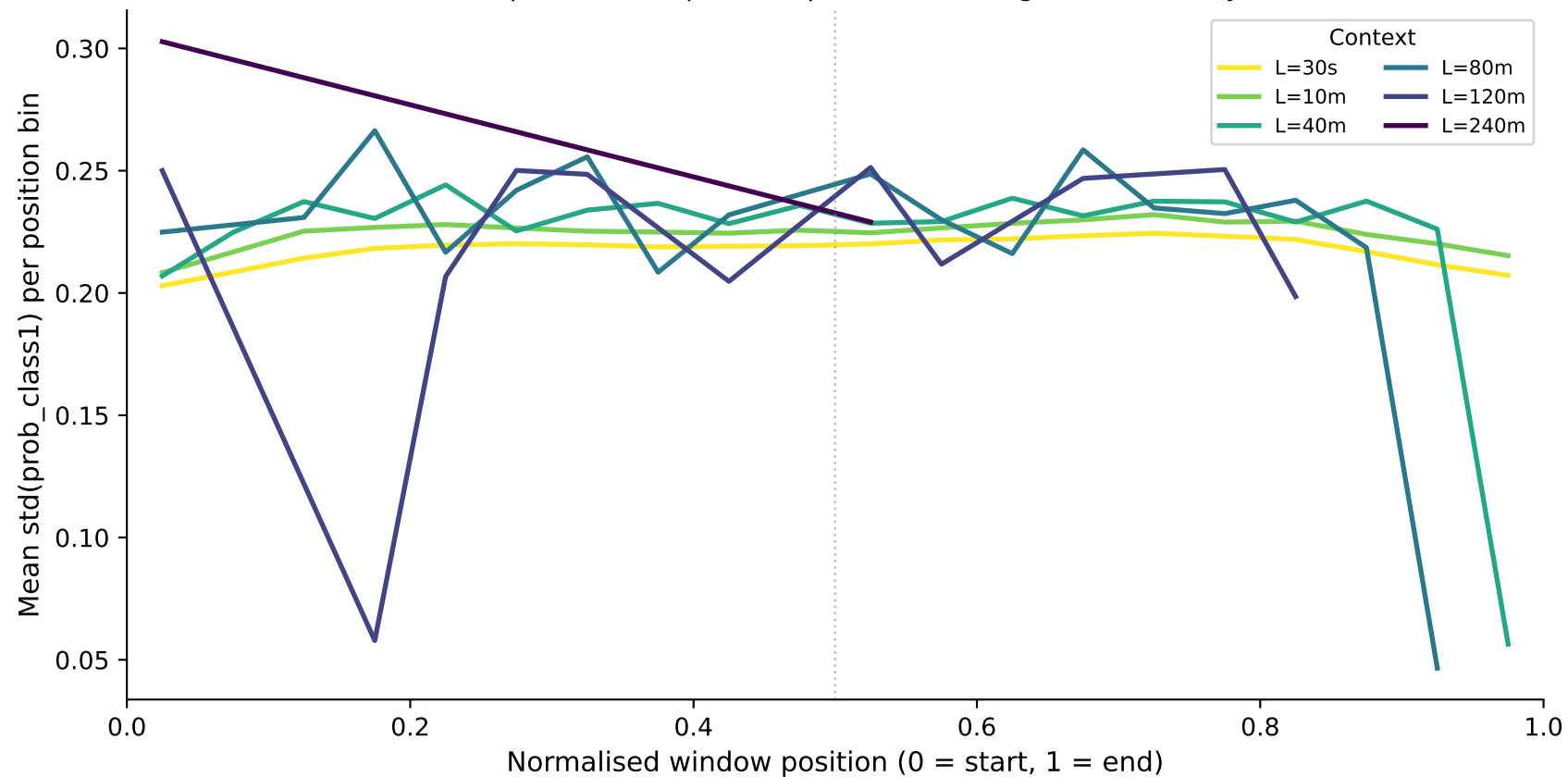
Prediction Variance vs Night Position — age_class (TRANSFORMER) Lower variance = position-independent predictions (longer context may flatten this)
