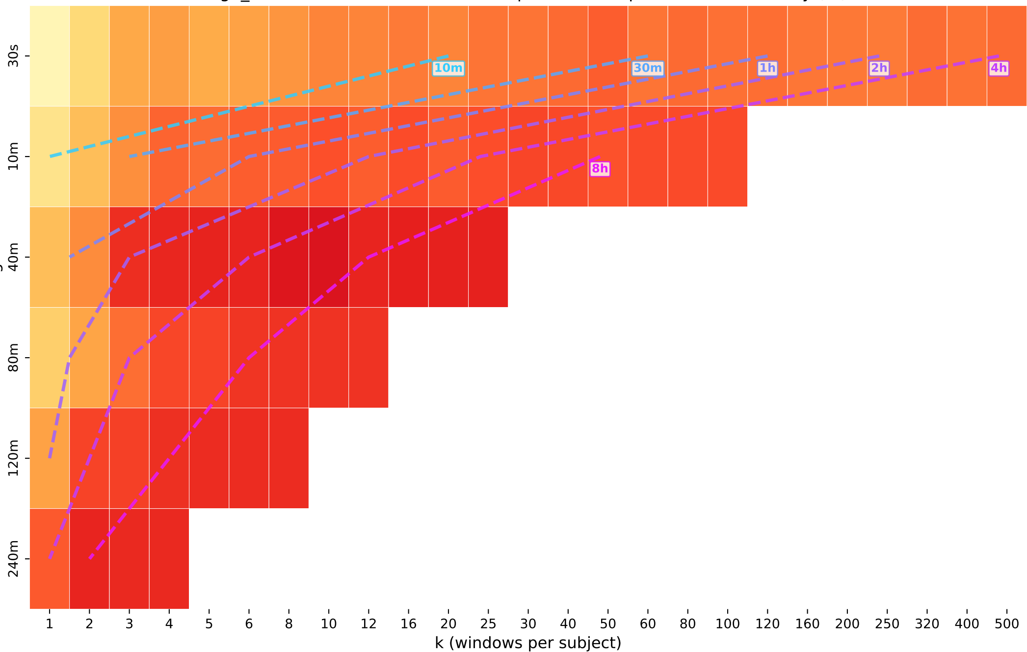
age_class · transformer — Iso-Compute Heatmap: Balanced Accuracy (%)
