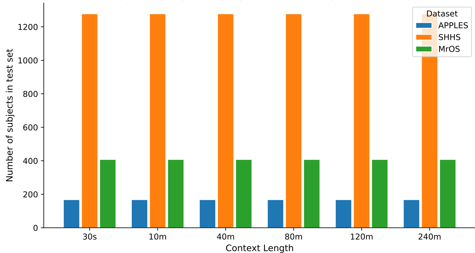
Test-Set Subject Count per Dataset — apnea_binary (LSTM) Subject count may drop at longer contexts (fewer qualifying windows)
