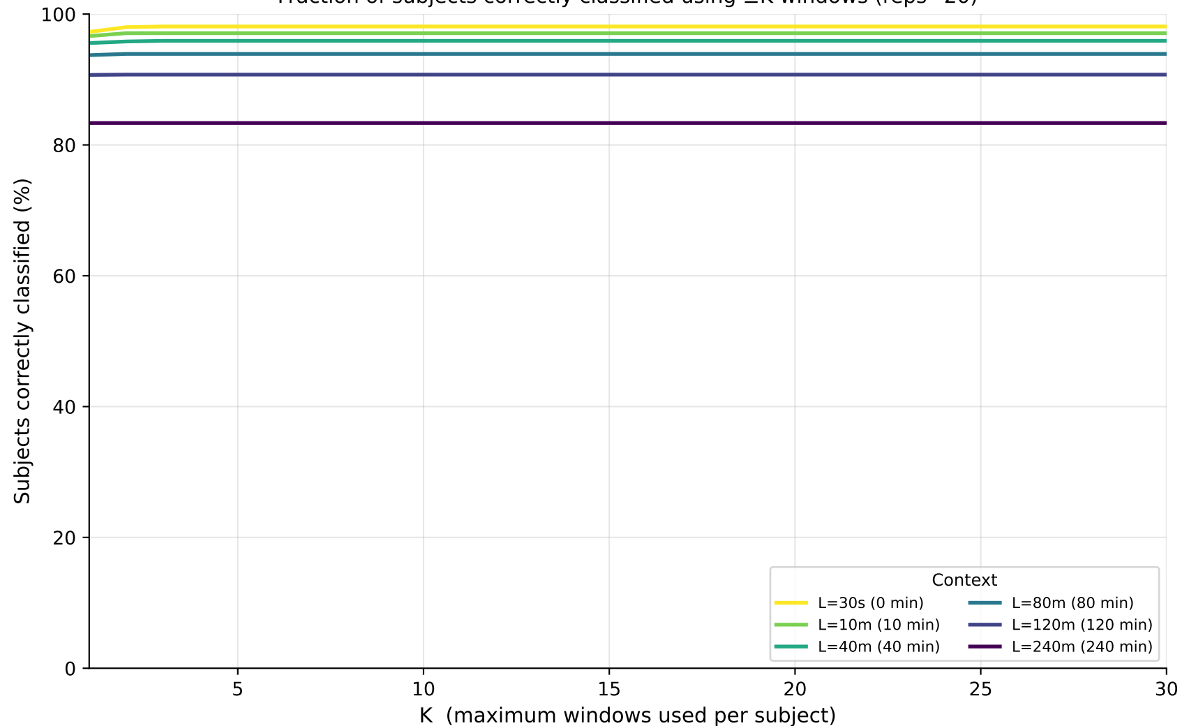
Coverage Curves — apnea_binary (LSTM) Fraction of subjects correctly classified using \leq K windows (reps=20)
