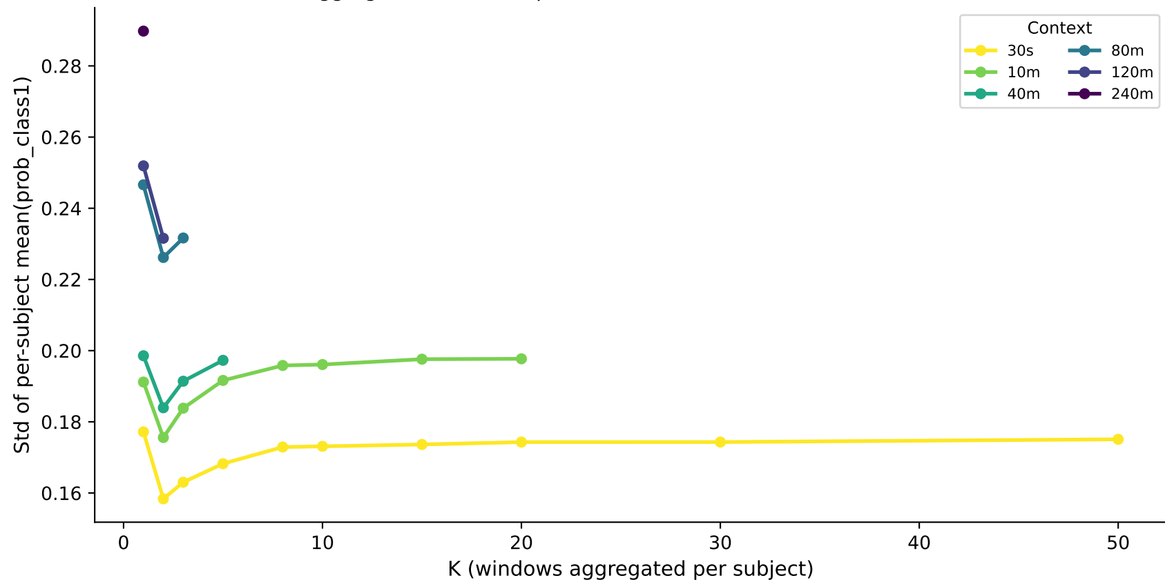
Prediction Variance vs K — apnea_binary (LSTM) Aggregation stabilises predictions (lower std = more consistent)
