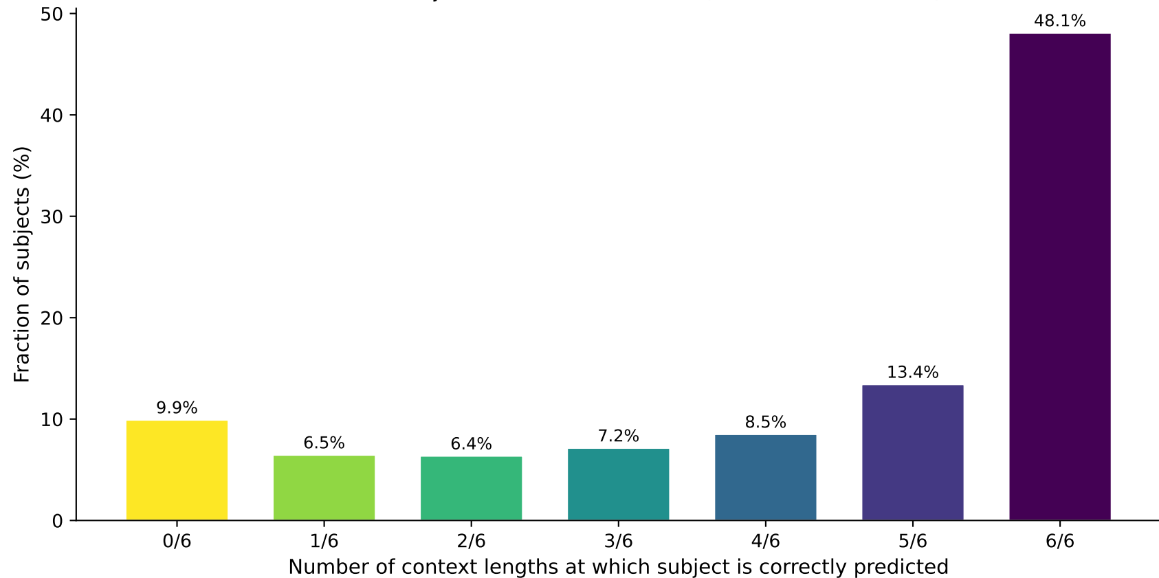
Hard-Subject Analysis — apnea_binary (LSTM) N = 2054 subjects · 0/6 = never correct (irreducible hard cases)
