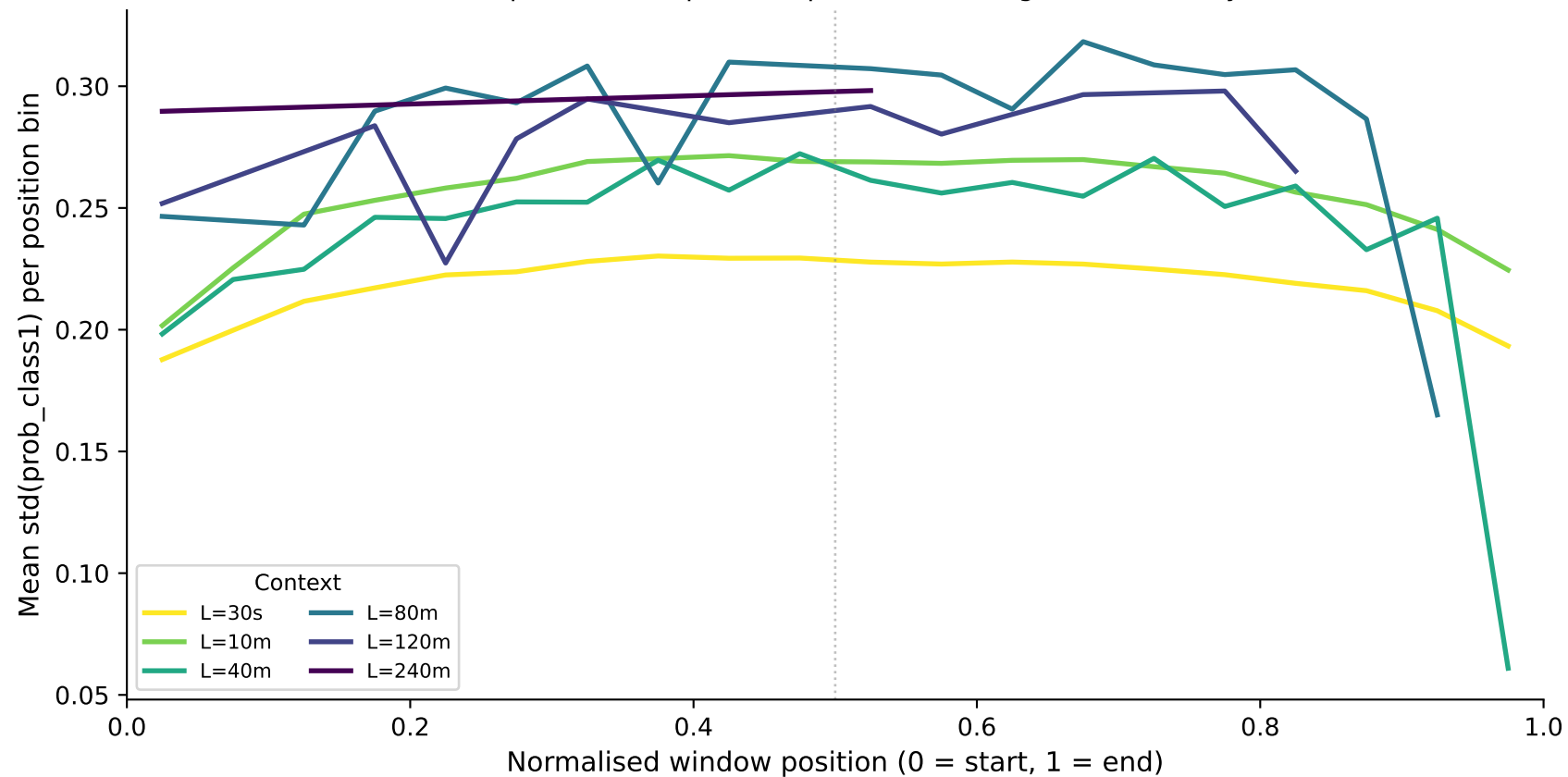
Prediction Variance vs Night Position — apnea_binary (LSTM) Lower variance = position-independent predictions (longer context may flatten this)
