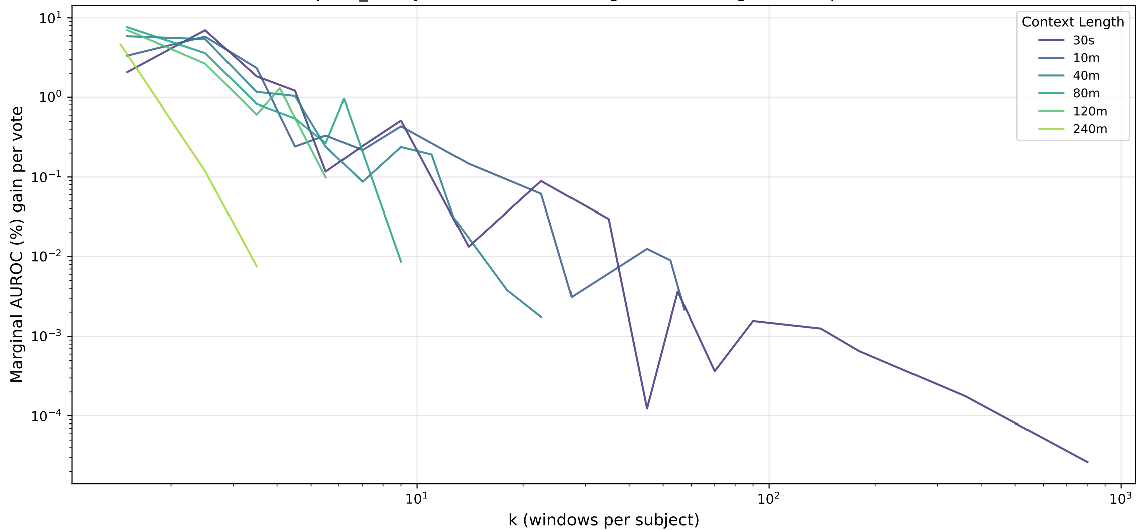
apnea_binary · lstm — Diminishing Returns: Marginal Gain per Vote
