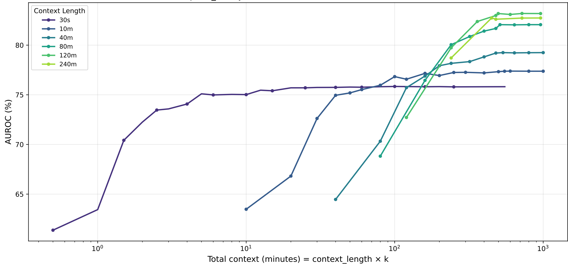
apnea_binary · lstm — AUROC (%) vs Total Context
