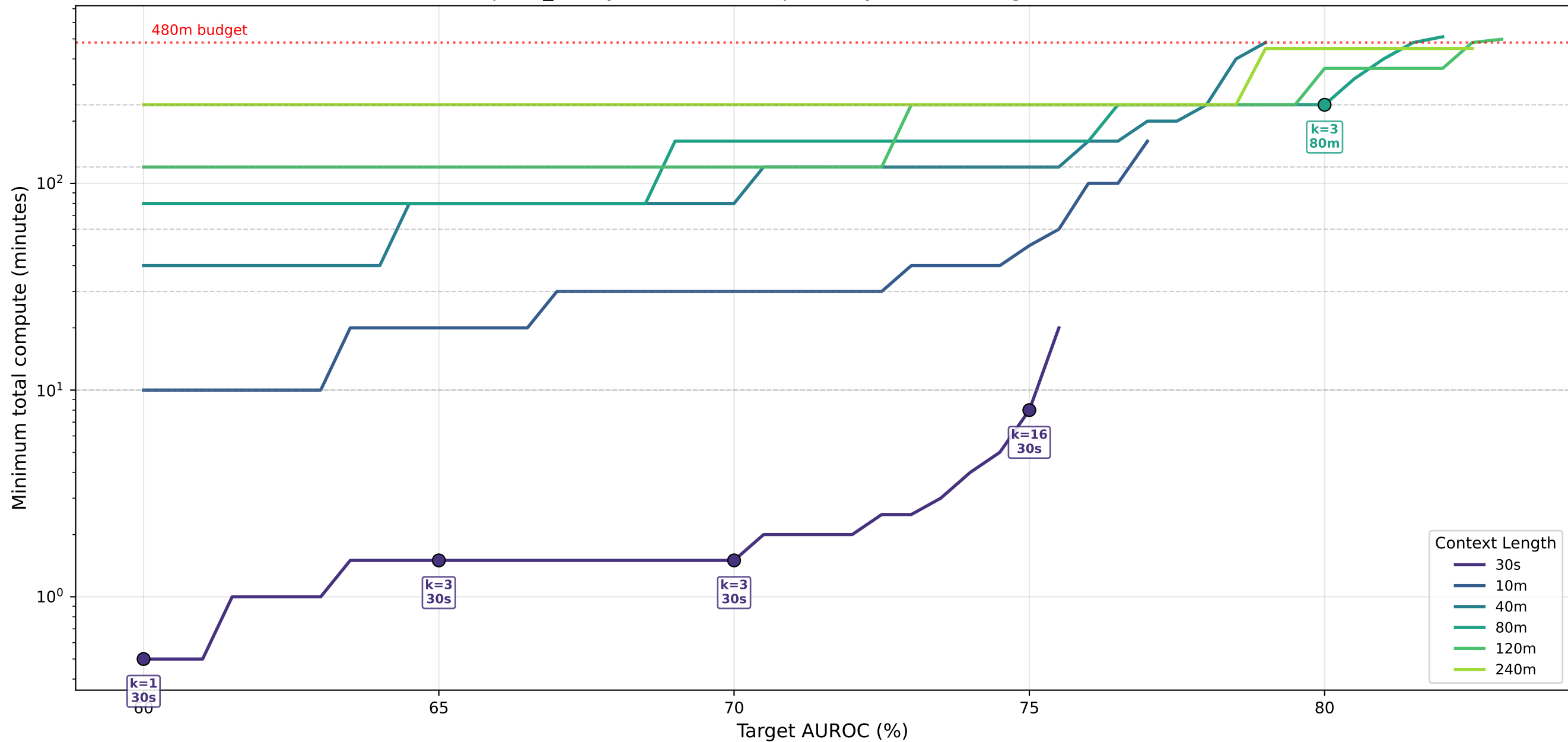
apnea_binary · lstm — Cheapest Way to Reach Target AUROC (%)
