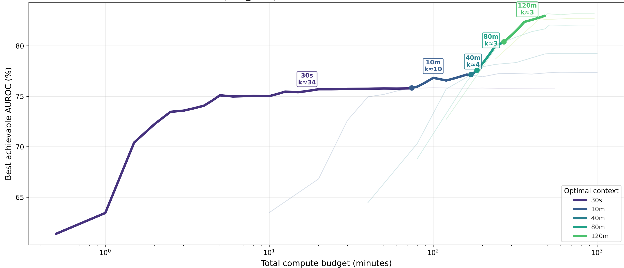
apnea_binary · lstm — Pareto Front: AUROC (%)
