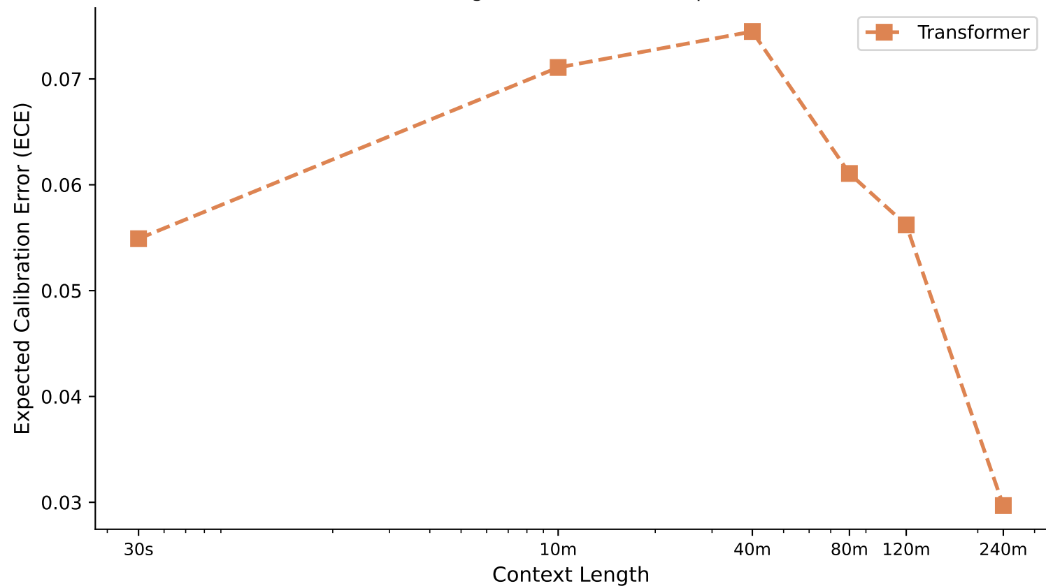
ECE vs Context Length — apnea_binary (K=10) Lower is better; longer context should improve calibration
