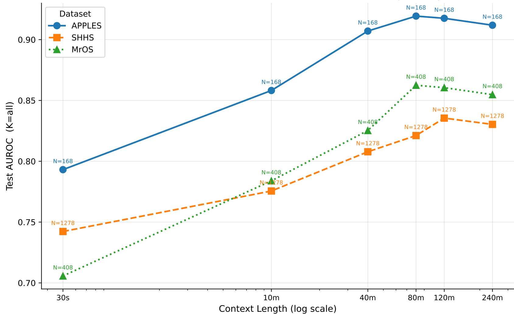
Cohort-Stratified Saturation — apnea_binary (TRANSFORMER) Does the context saturation result hold across each dataset independently?
