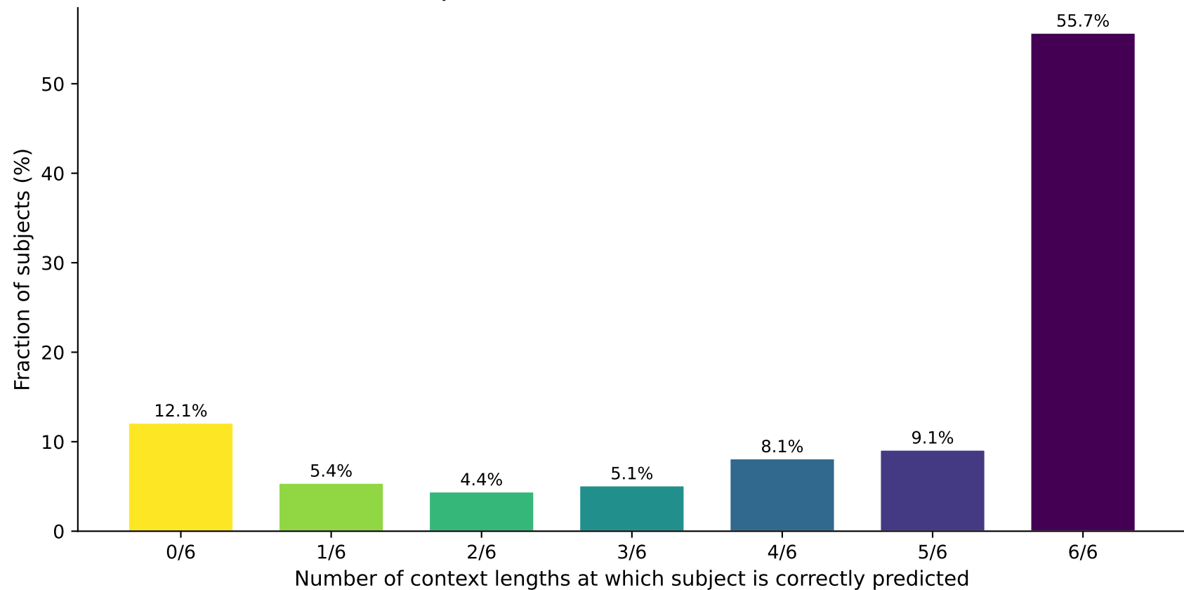
Hard-Subject Analysis — apnea_binary (TRANSFORMER) N = 2054 subjects · 0/6 = never correct (irreducible hard cases)
